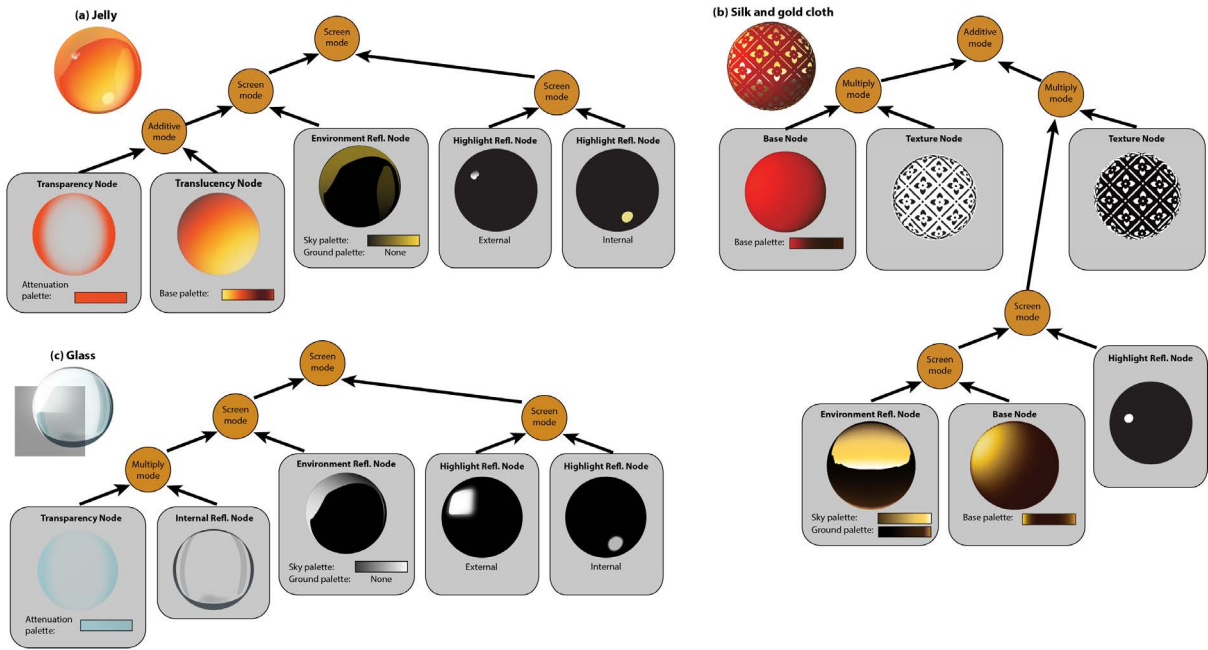
Figure 2.15: Vector Shade Trees for three materials: jelly, silk and gold cloth and glass, obtained by combining nodes for transparency, translucency, reflections, highlights, textures, base shading. Each node generates vector shapes filled with color gradients. (Lopez-Moreno et al. 2013)
