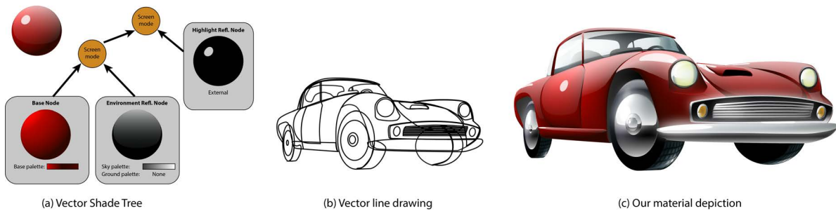
Figure 2.5: A Vector Shade Tree represents a stylized material by combining basic shading nodes (a). By assigning various shade trees to the regions of a line drawing (b), users can quickly colorize vector illustrations with rich material appearance (c). (Lopez-Moreno et al. 2013)
