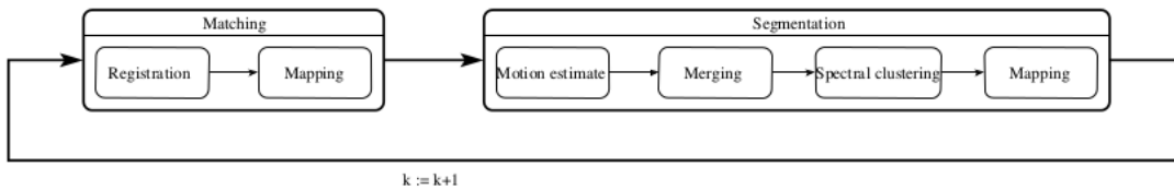
Figure 3.9: Overall pipeline of our algorithm, at iteration k , 1 \leq k < f . As input we have meshes M^k , together with an initial segmentation estimate \Sigma_{est}^k and M^{k+1} . As output we get a segmentation \Sigma^k of M^k and an initial segmentation estimate \Sigma_{est}^{k+1} of M^{k+1} .
