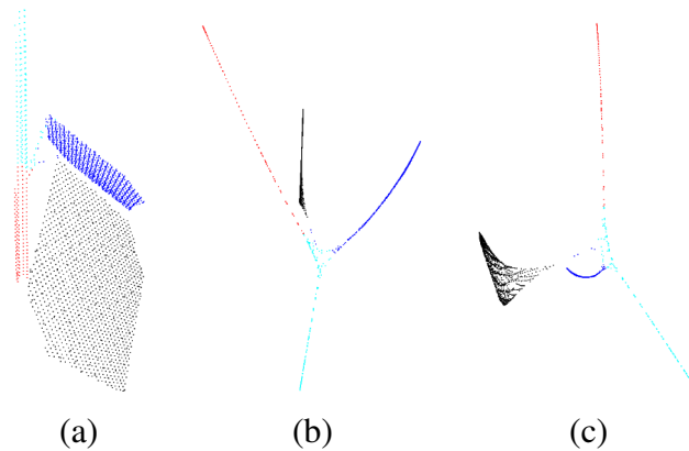
Figure 4.5: (b,c) Two views of the spectral embedding of the point cloud shown in (a).
