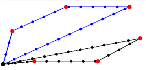
Figure 8.5: C_{max,i} = 3 , C_{max,-i} = 3
