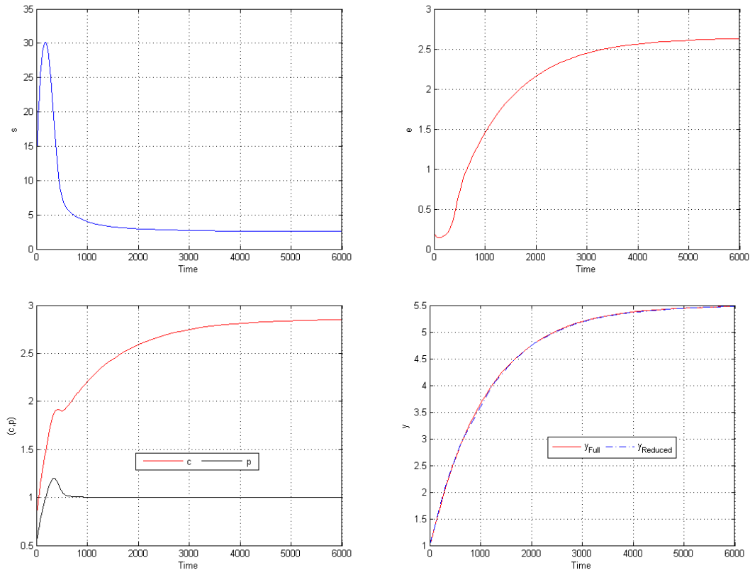
FIGURE 2.7.5: Taking these values of parameters k_{-2} = 0.2, k_{-1} = 0.3, k_1 = 0.2, k_2 = 0.36, k = 0.5, k_e = 0.005, \gamma_e = 0.0009, \theta_p = 0.4, s(t_0) = 12, e(t_0) = 0.2, c(t_0) = 0.8, p(t_0) = 1, y(t_0) = 1, u = 0.5 , in the beginning of the simulation we have u > k_2 y(0) , therefore first the equilibrium of the fast system does not exist; then the substrate s start increasing and because we have the production of the enzyme by the gene ( p > \theta_p ) it turns that u < k_2 y(t) and finally the substrate s converges to the equilibrium.
