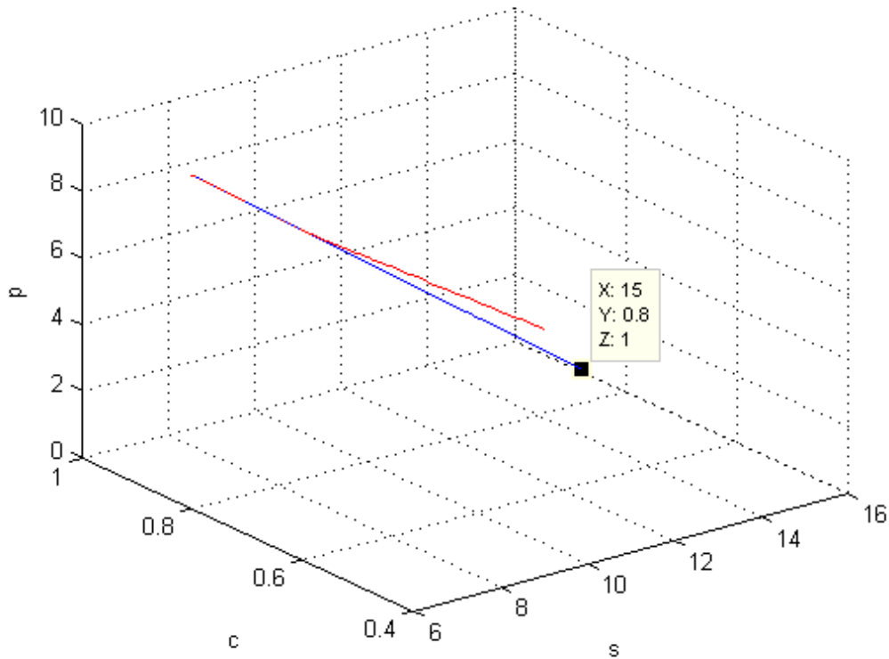
FIGURE 2.2.2: Simulations of system (2.2.2) with two different initial conditions starting from the same hyperplane (s_{01} = 15, c_{01} = 0.8, p_{01} = 1) , (s_{02} = 9, c_{02} = 0.4, p_{02} = 7.4) and with the parameters k_{-2} = 0.2, k_{-1} = 0.3, k_1 = 0.2, k_2 = 0.5, E_0 = 1 .
