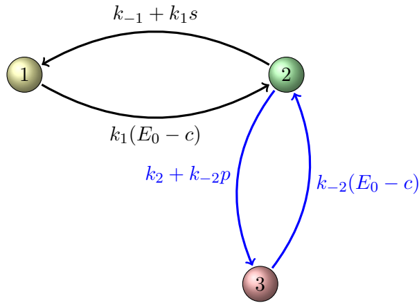
FIGURE 2.2.1: Graph of the Jacobian matrix is strongly connected
