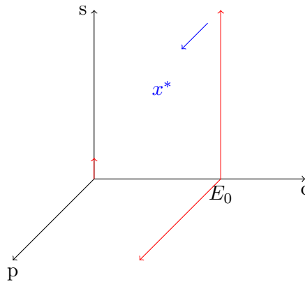
FIGURE 2.3.3: The vector fields in the upper and lower vertices of the hyperrectangle.
