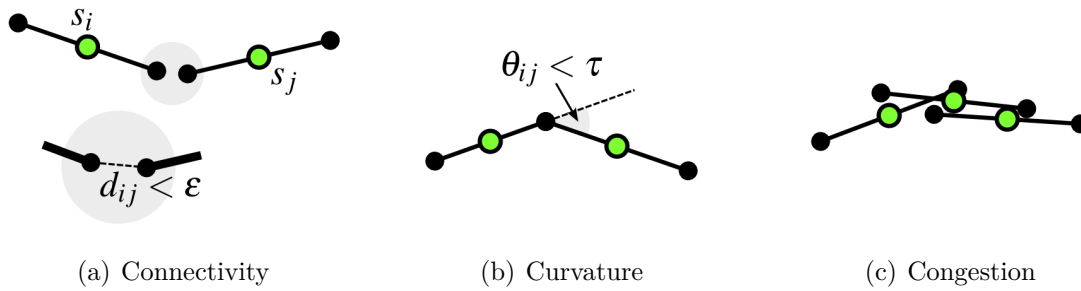
Figure 2.7: Stochastic models constrain the spatial distribution of the line segments, where each line segment s_i is represented as a tuple of its center coordinate \mathbf{x}_i , length l_i , and orientation \theta_i . (a) Pair line segments are assumed to be connected if the end-to-end distance d_{ij} of them is relatively small ( < \epsilon ). (b) The angular difference \theta_{ij} of two line segments is related to the curvature. A small curvature is preferred in order to reconstruct smoothly connected curvilinear structures. (c) Congestion of line segments will be penalized.
