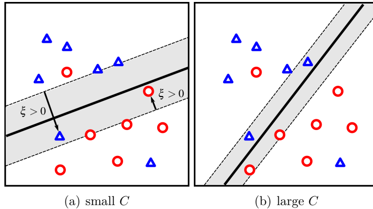
Figure 4.4: For the given linearly non-separable data points, we employ soft margin SVM which allows small classification errors around margin. A slack variable measures the such violation on the marginal areas. We modify the objective function of SVM to take into account the amount of margin violation with a parameter C . The hyperplane on the left figure is obtained using a small C so that it is less sensitive for classification errors and margin violations. On the other hand, the hyperplane on the right figure is more strict with respect to the margin violation by employing a larger C value.
