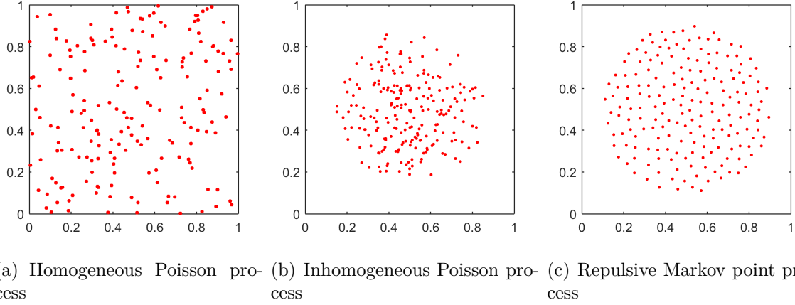
Figure 3.2: Comparison with the realization of point patterns obtain by (a) homogeneous Poisson process, (b) inhomogeneous Poisson process, and (c) repulsive Markov point process. For a finite space, homogeneous Poisson process employs a constant intensity measure, whereas inhomogeneous Poisson process employs intensity measure as a function. Both Poisson processes ignore correlation of points in the space. On the other hand, Markov point process constrains the local interaction of neighboring points using a non-negative density function. Here, repulsive constraint prevents overlapping between points.
