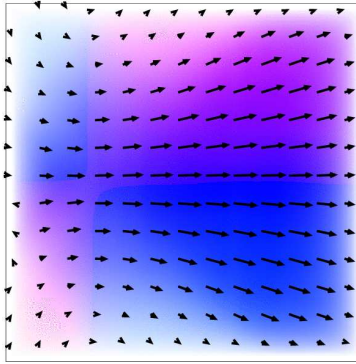
Figure 4.5 – Estimation result \mathbf{w}_{\mathcal{M}_2}(0) .
