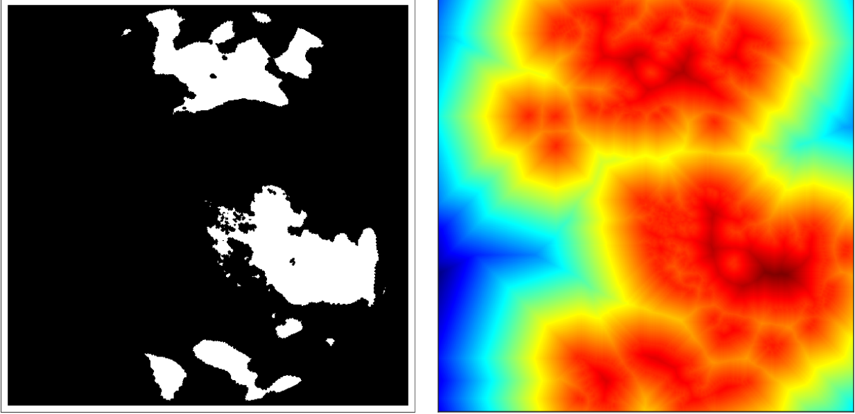
Figure 2.3 – Threshold of the precipitation rate ( on the left ) and the signed distance map to the structures ( on the right ).
