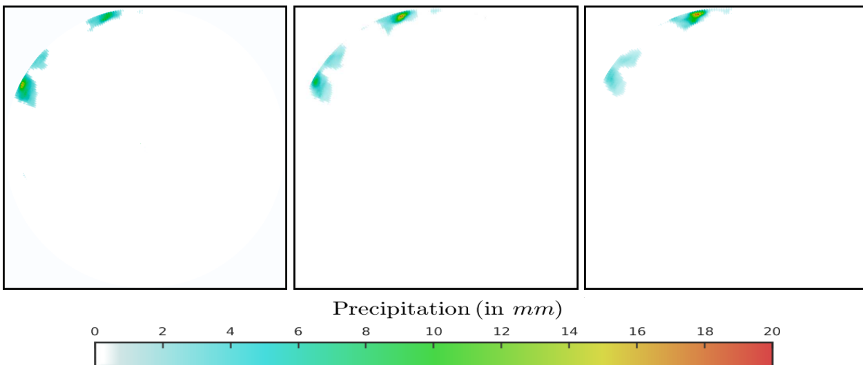
Figure 4.16 – Observations \mathbf{Y}_1, \mathbf{Y}_2 and \mathbf{Y}_3 .
