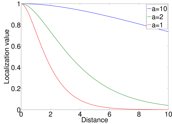
Figure 6.4: Values of \rho_d , for a_d = 1, 2, 10 , as a function of the distance between pixels.
