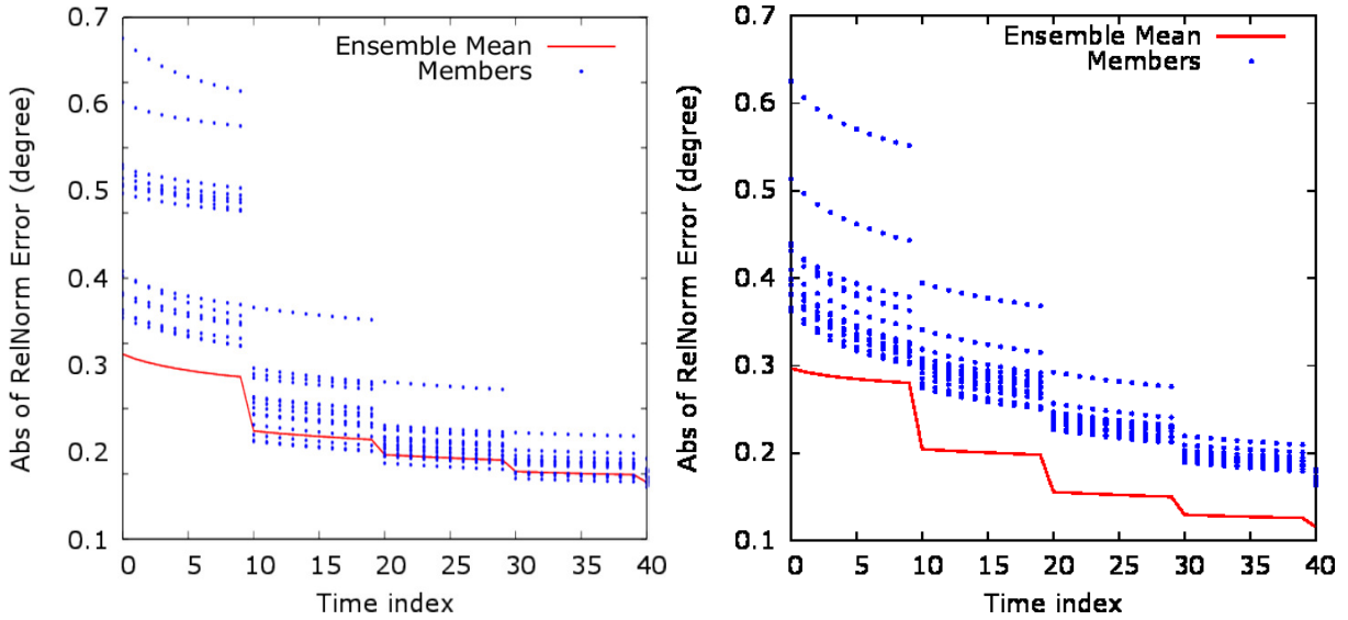
Figure 8.4: Values of the relative norm error without localization ( left ) and with localization ( right ).
