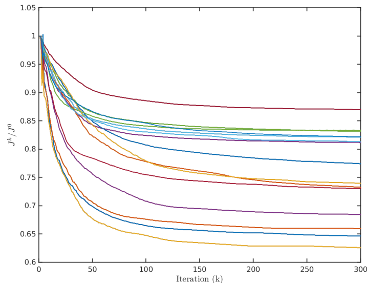
Figure 1.3: Values of the cost function at iteration k divided by the one at initialization, depending on the number of iterations during the minimization. Each curve corresponds to a different experiment.
