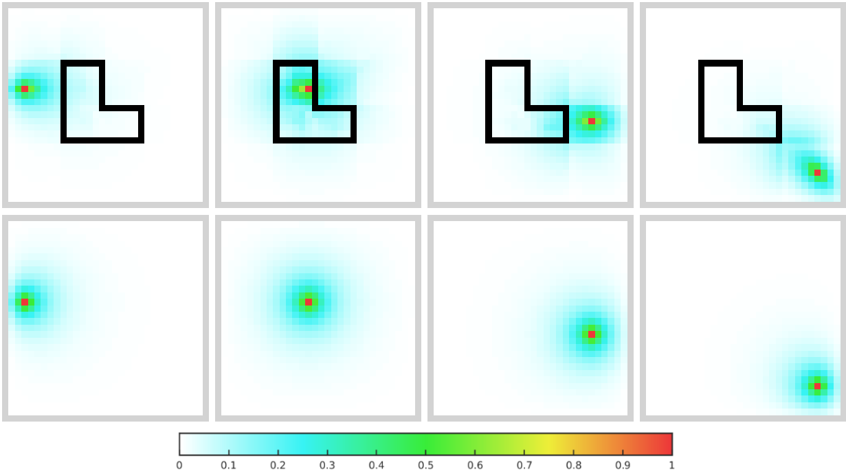
Figure 3.2: Covariance values computed between the red pixel and the rest of the domain with both \mathcal{R}_1 and \mathcal{R}_4 (top line), with only \mathcal{R}_1 (bottom line). The black curve is used to determine d(\mathbf{p}) .
