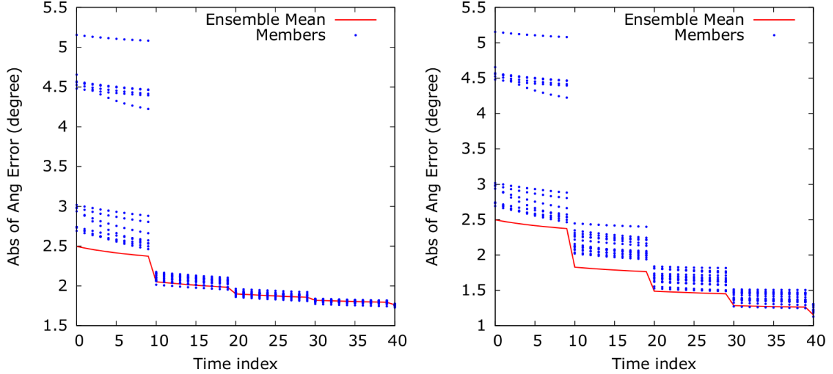
Figure 8.3: Absolute values of the angular error without localization ( left ) and with localization ( right ). The blue points correspond to one member of the ensemble and the red curve to the ensemble mean.
