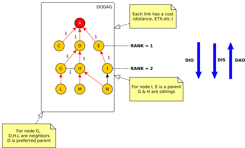
Figure 2.15: RPL DODAGs.
