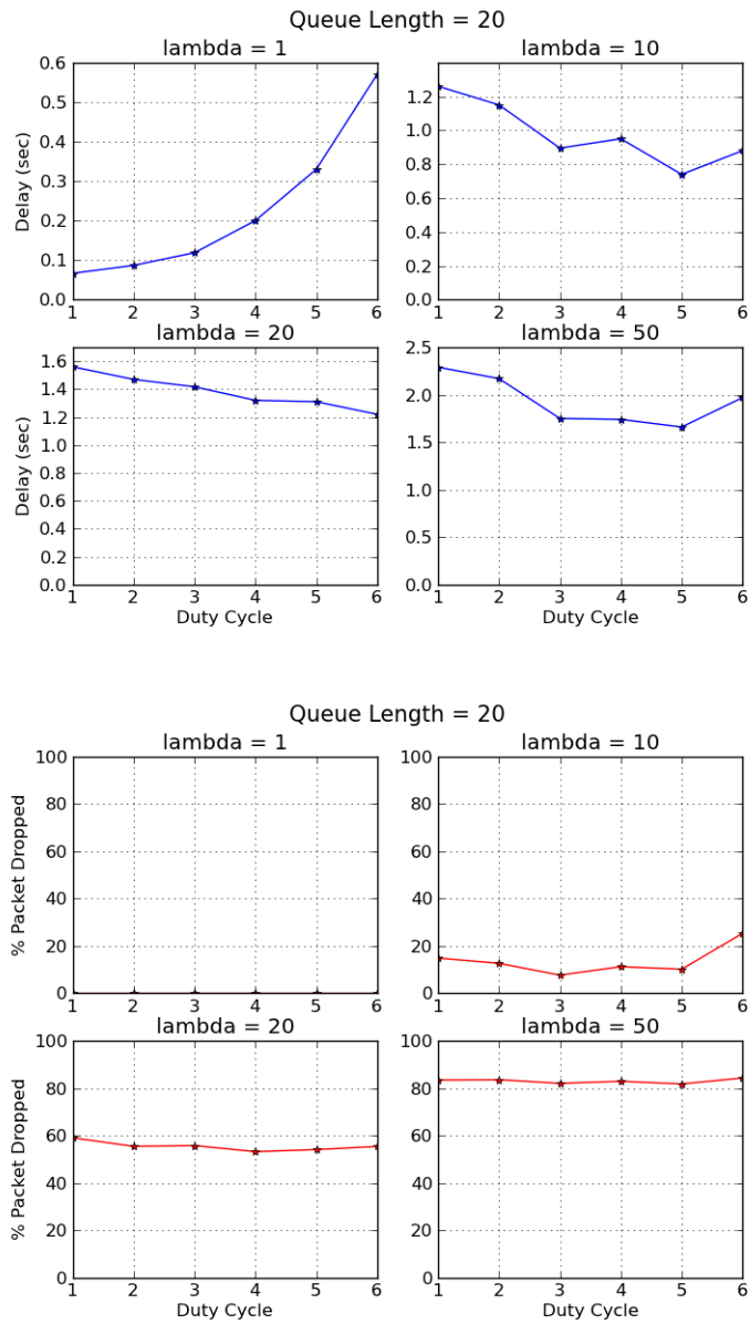
Figure 4.10: Duty Cycle = 50%, Buffer Length = 20.
