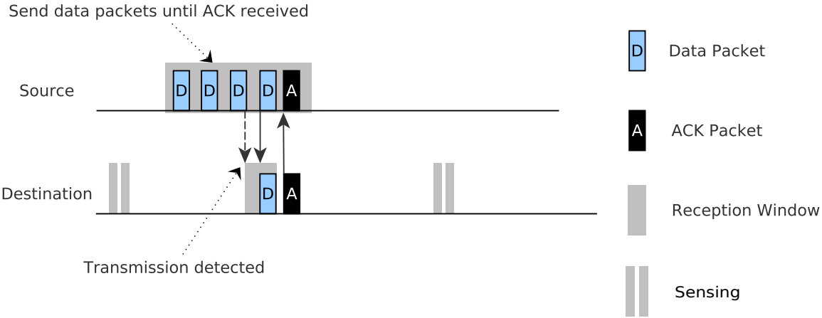
Figure 2.12: ContikiMAC mechanism.
