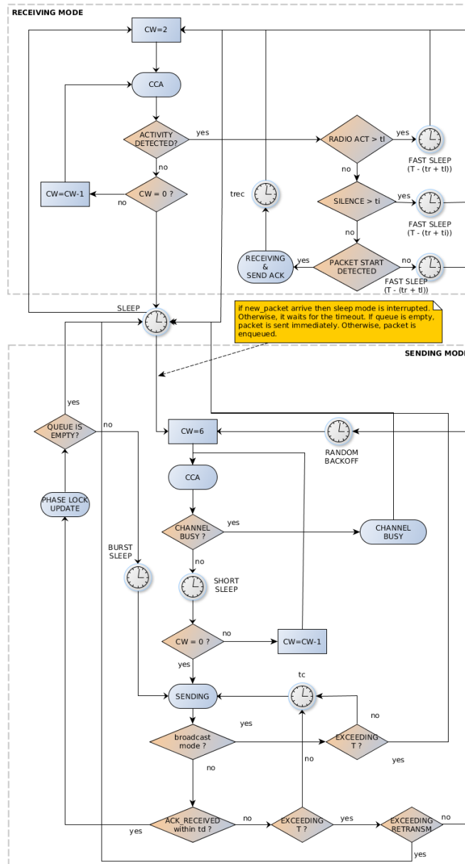
Figure 5.8: ContikiMAC flow diagram.
