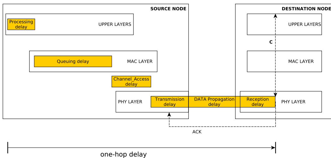
Figure 2.1: One hop delay components.
