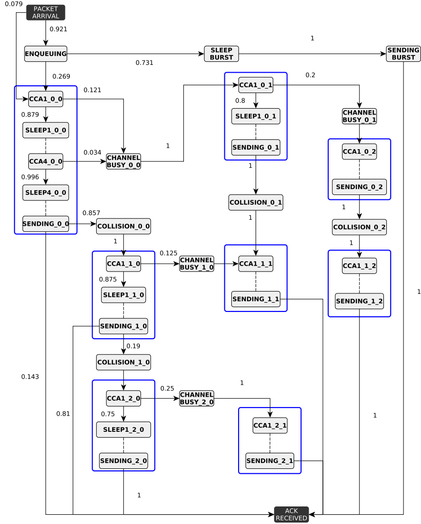
Figure 5.10: Obtained Markov chain for a single device.
