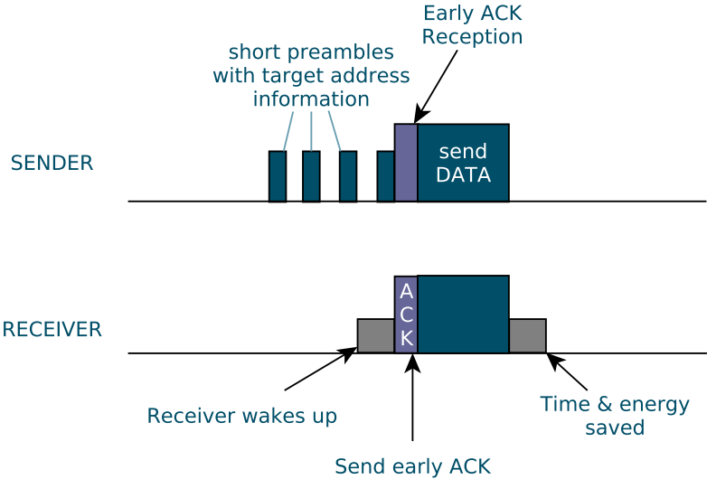
Figure 2.11: X-MAC short preamble approach.
