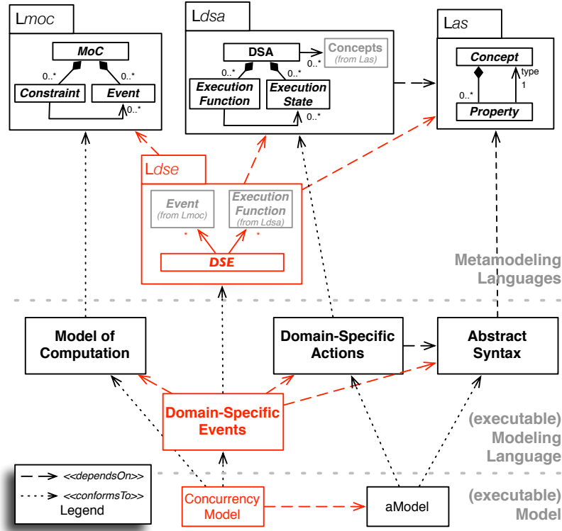
Figure 2.6: Modular design of a concurrency-aware xDSML
