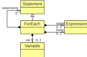
Figure 3.2: foreach loop in ORCC IR
