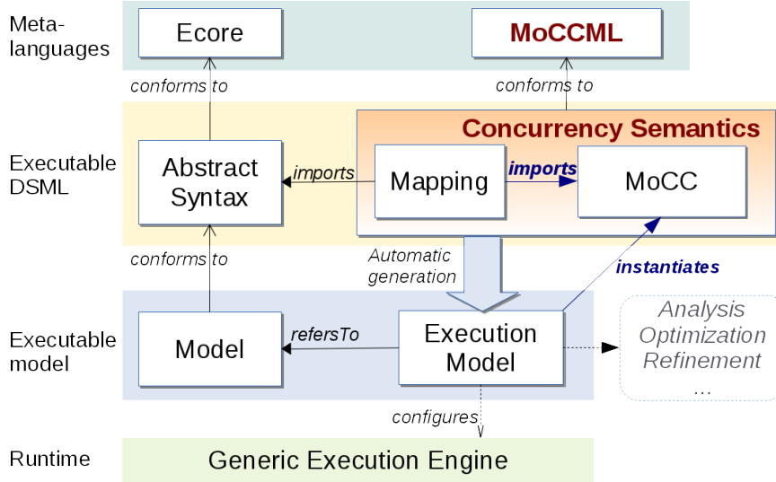
Figure 2.7: Big picture of MoCCML
