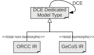
Figure 3.5: Total subtyping
