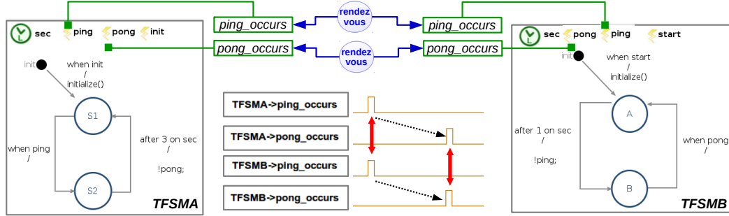
Figure 3.20: Application of the synchronized product operator on two TFSMs
