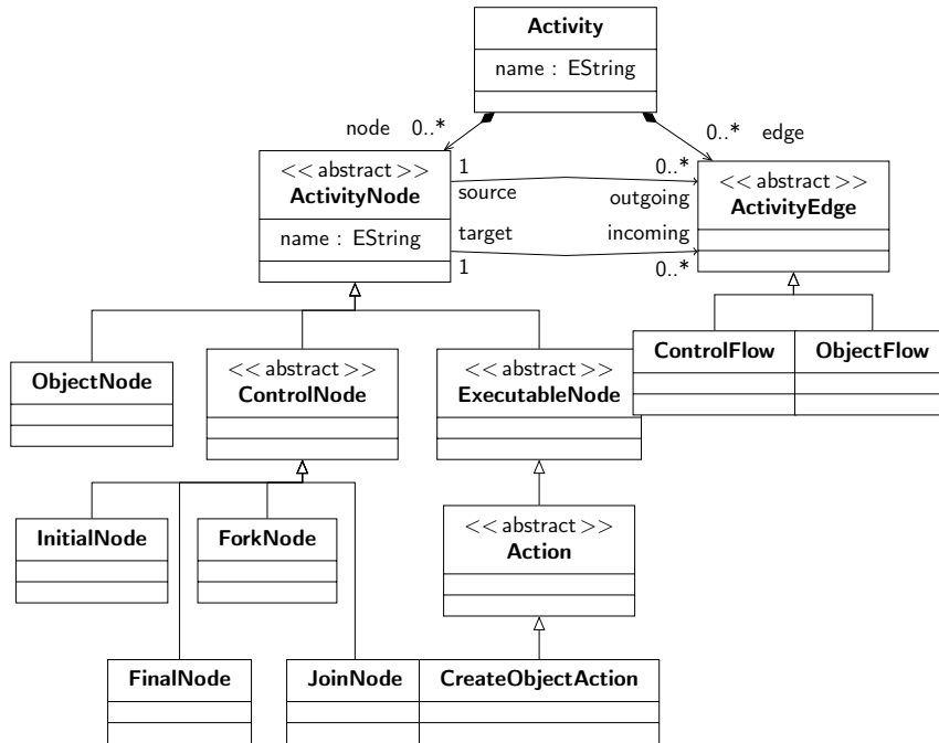
Figure 2.1: Excerpt of the fUML Metamodel
