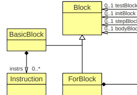
Figure 3.3: for loop in GeCoS IR
