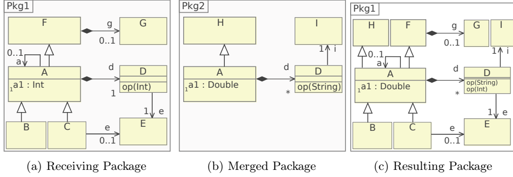
Figure 3.12: Merge Operator
