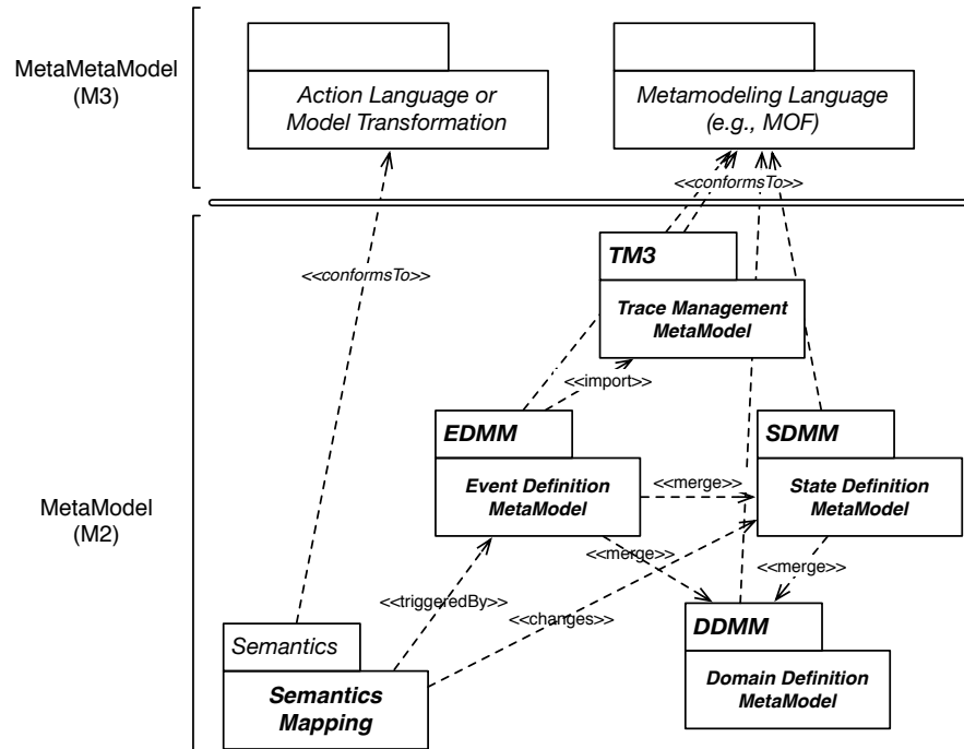
Figure 2.4: The xDSML pattern
