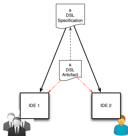
Figure 5.2: Metamorphic DSL (abstract scenario)
