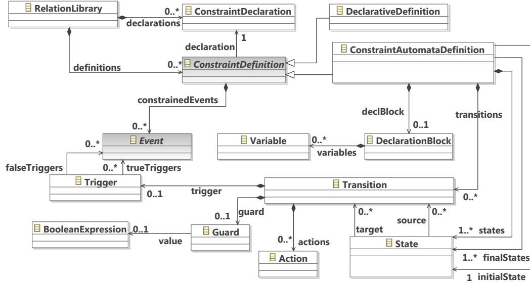
Figure 2.8: Excerpt of the MoCCML metamodel
