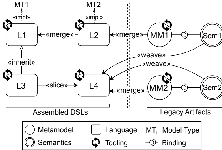
Figure 3.10: DSMLs Assembly and Customization with Melange
