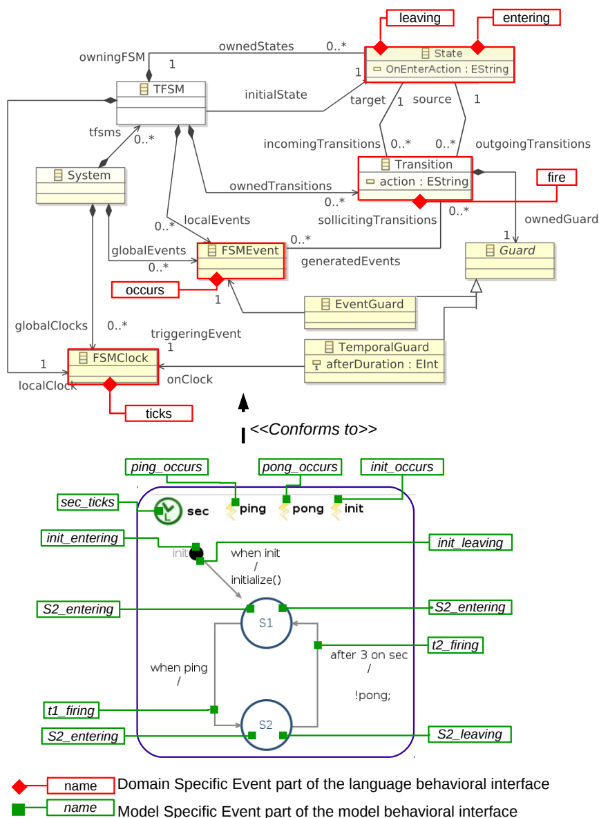
Figure 3.18: A TFSM metamodel (top) and a conforming model (bottom) with their respective behavioral interfaces
