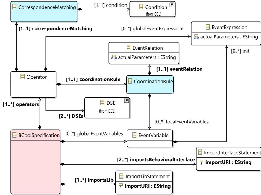
Figure 3.19: Excerpt of the B-COOL metamodel
