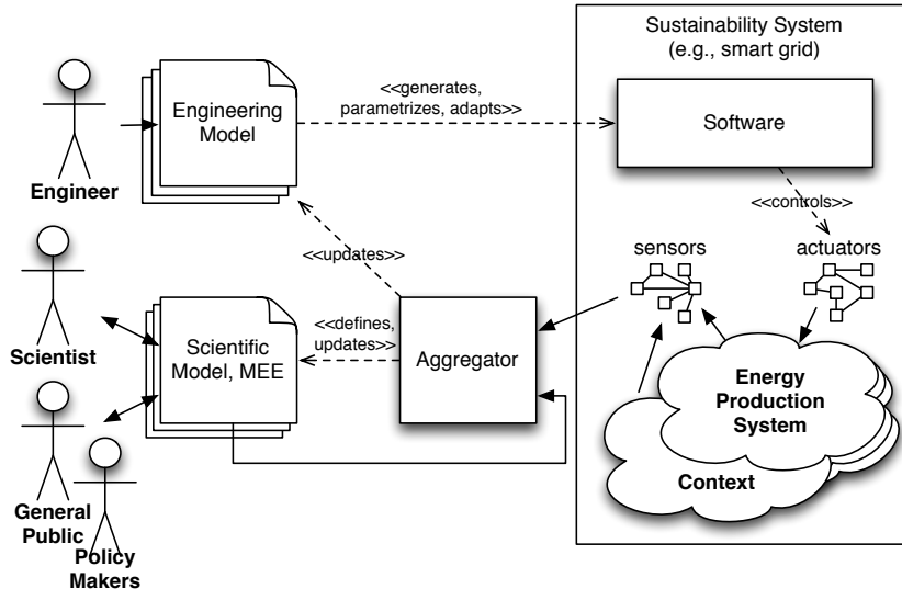
Figure 5.4: Intertwined use of engineering and scientific models
