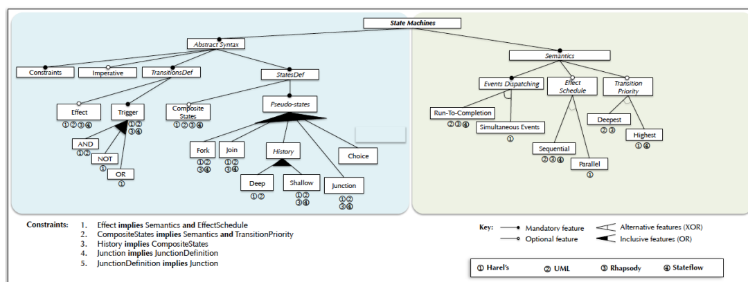
Figure 3.16: Feature model of the family of DSMLs for Finite State Machines
