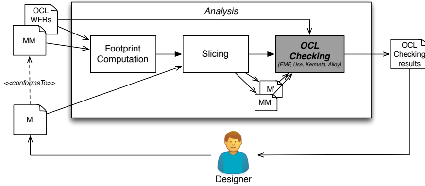
Figure 2.3: Approach overview
