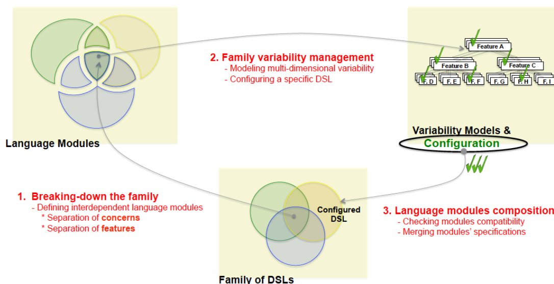
Figure 3.15: Approach overview for variability management in DSMLs
