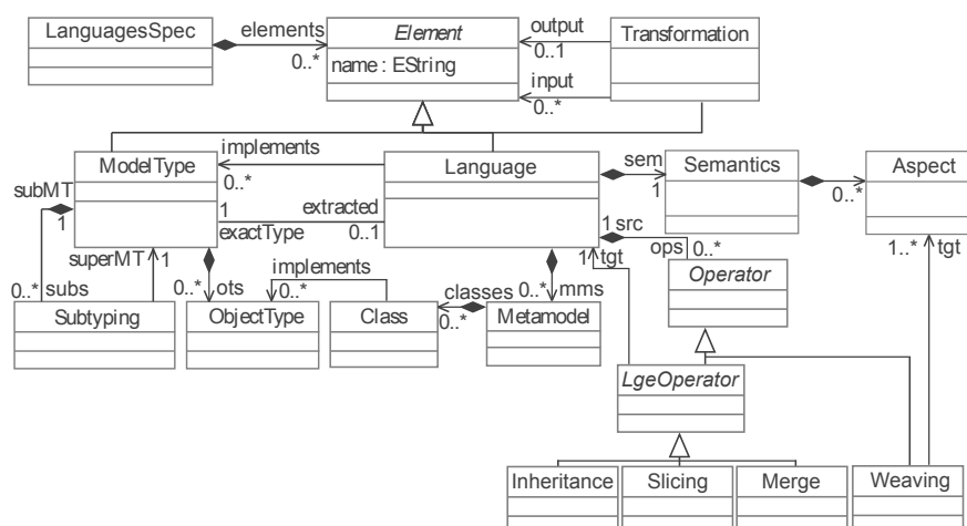
Figure 3.14: Excerpt of the abstract syntax of Melange
