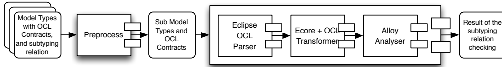
Figure 3.8: Contract Matching Checking Tool Overview
