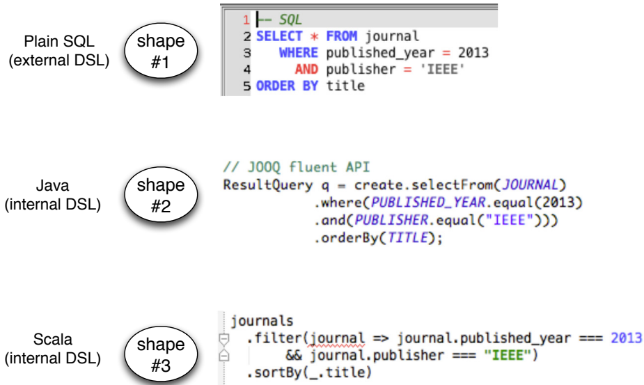
Figure 5.1: Three SQL shapes : plain SQL, JOOQ fluent API in Java, Slick API in Scala
