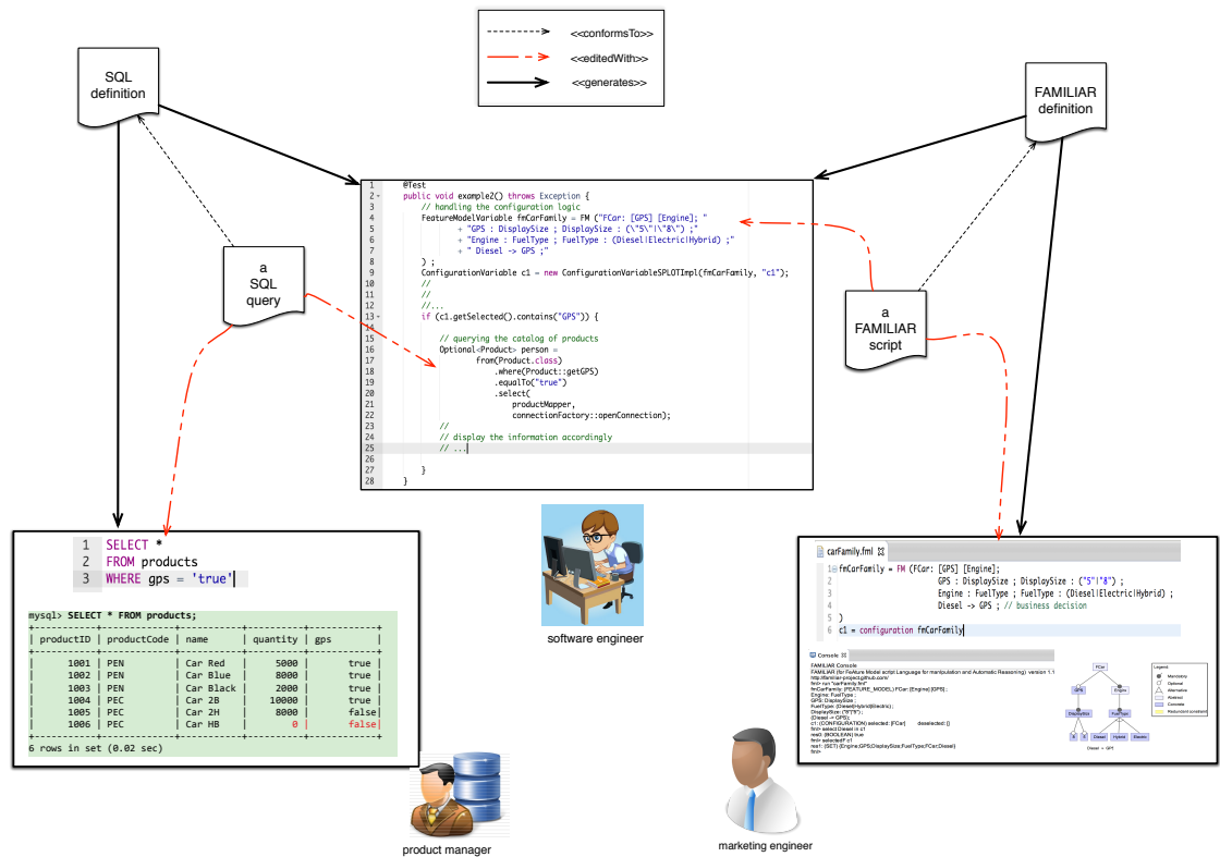
Figure 5.3: Metamorphic DSL (concrete illustration)
