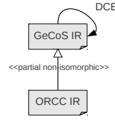
Figure 3.6: Partial non-isomorphic subtyping
