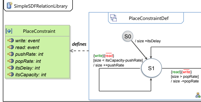
Figure 2.9: Screenshot of the MoCCML graphical editor
