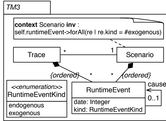
Figure 2.5: A simplified TM3 for Discrete-Events Modeling
