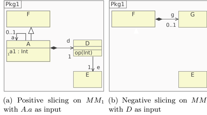
Figure 3.13: Examples of metamodel slices
