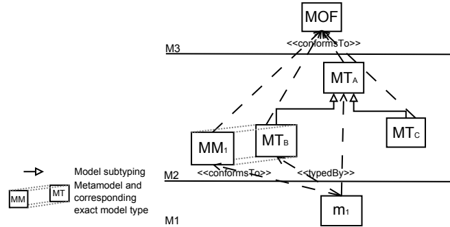
Figure 3.1: Conformance, model typing and model subtyping relations
