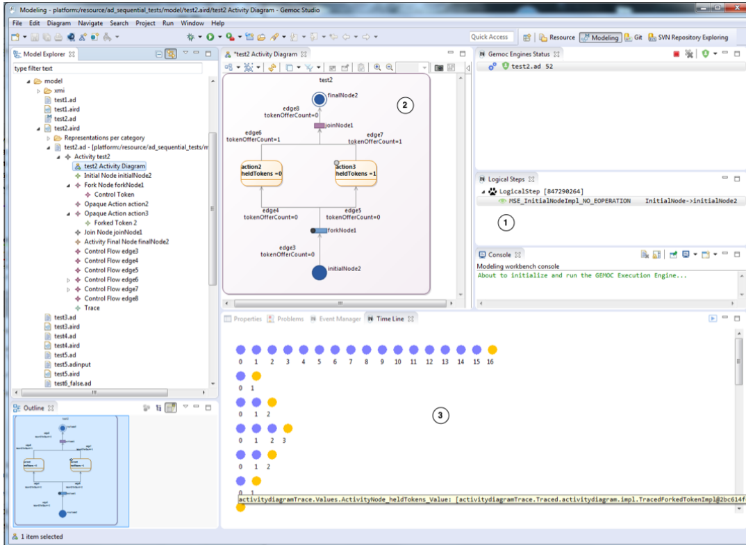
Figure 2.10: Resulting modeling workbench for UML Activity Diagram
