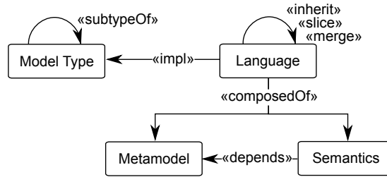
Figure 3.11: Model Typing Relations
