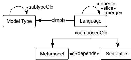
Figure 3.11: Model Typing Relations
