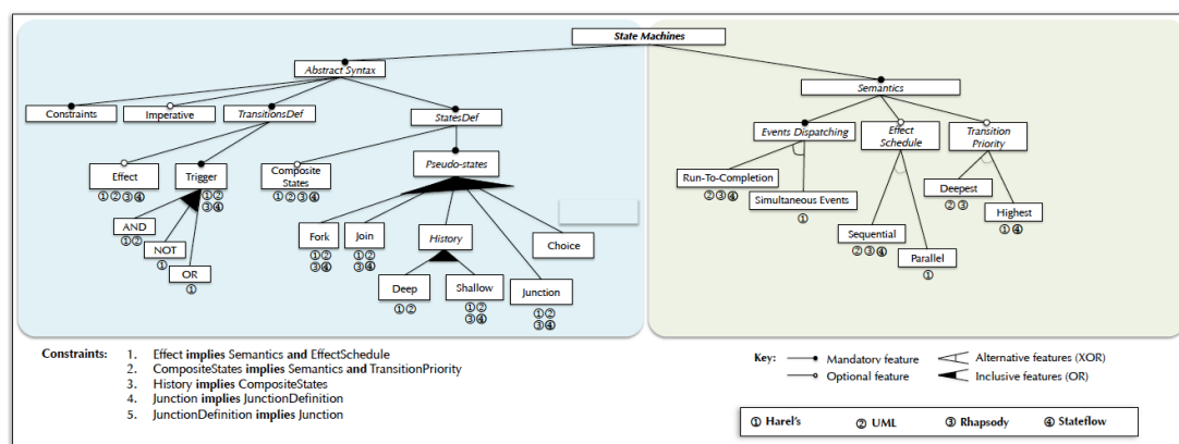
Figure 3.16: Feature model of the family of DSMLs for Finite State Machines
