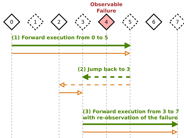
(b) Reconstruction-based omniscient debugging scenario, with a trace containing half of the states.
