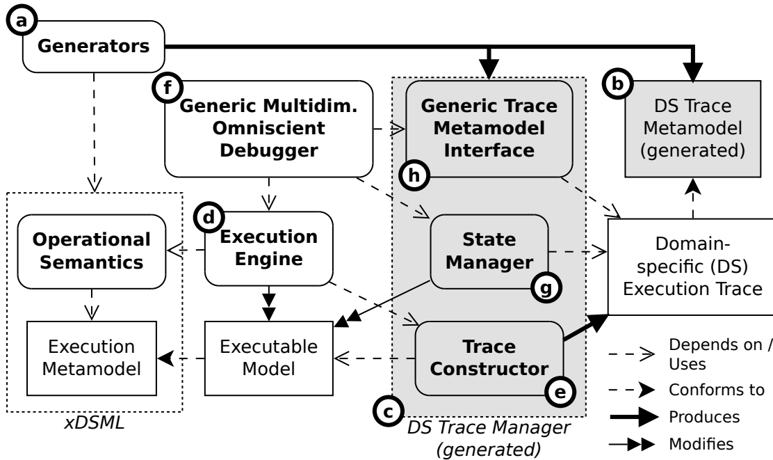
Figure 8.3: Overview of the advanced and efficient omniscient model debugging approach.
