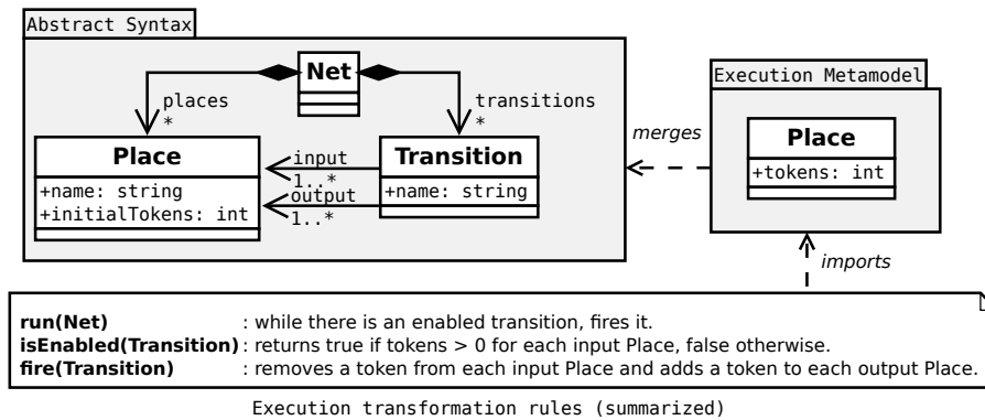
Figure 5.1: Petri net xDSML (reminder from Chapter 2).
