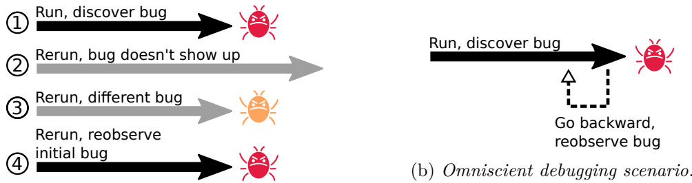
(a) Cyclic debugging scenario using interactive debugging.
