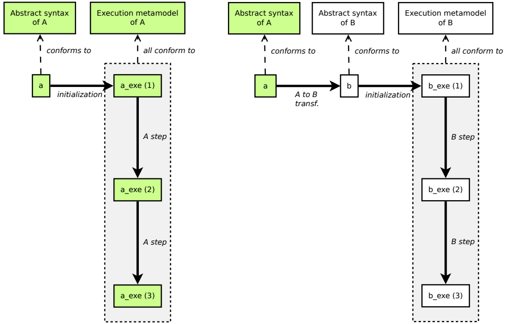
(a) Operational semantics. (b) Translational semantics, using a target xDSML B.
