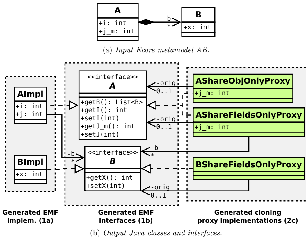
Figure 9.2: Example of implementation classes after calling both the EMF code generator and our cloning material generator on the metamodel AB.
