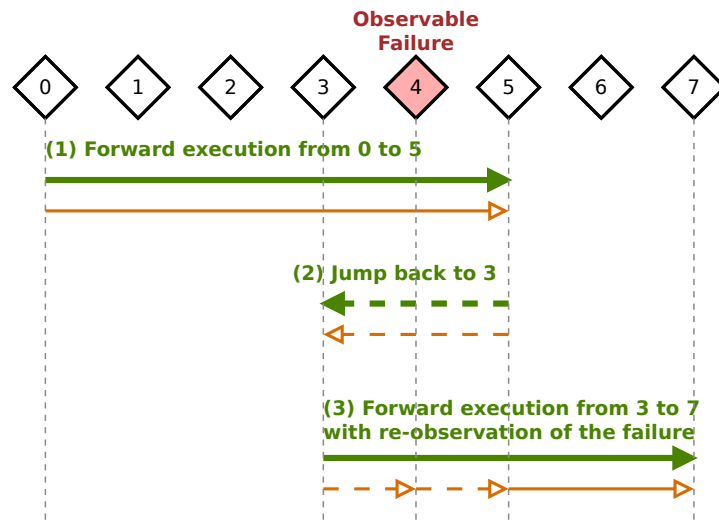
(a) Trace-based omniscient debugging scenario, with a trace containing all states.
