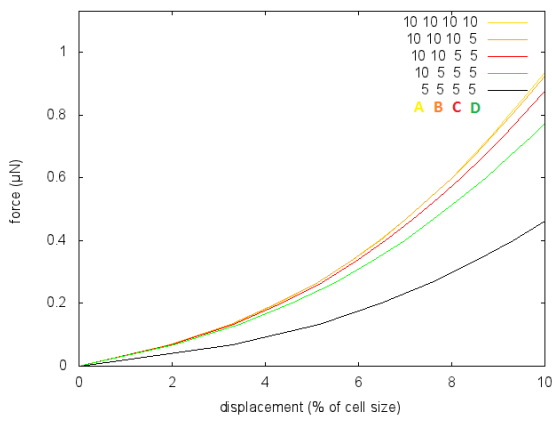
(b) P = 0 , different elastic modulus, indentation in the cell middle
