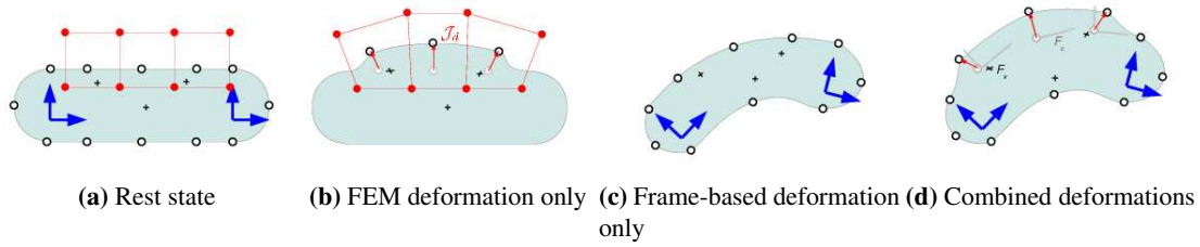
FIGURE 4.3 – Example of a two-level MHMM, using a frame-based coarse model (blue) and an FEM detail model (red). The detail displacements \mathcal{J}_d (4.3b) are applied in local frames defined by the deformation gradients \mathcal{F}_c of the coarse displacements (4.3c) to generate the combined deformations (4.3d).
