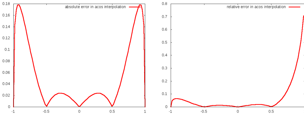
(a) absolute error of interpolation of arccos with La- (b) relative error of interpolation of arccos with La- grange method grange method
