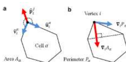
FIGURE 1.8 – Example of forces acting on vertices in a vertex based model (source [Fletcher et al., 2014])
