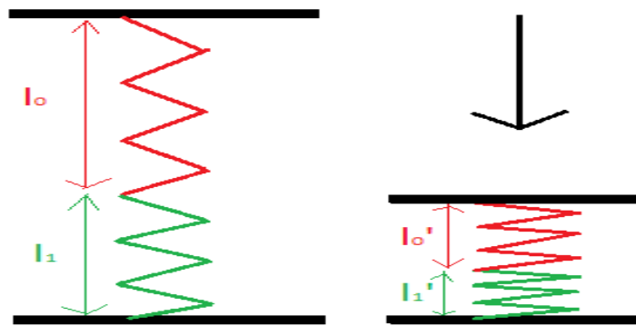
FIGURE 2.18 – Principle of the method : observation of 2 springs in series undergoing a known displacement yields stiffness ratios
