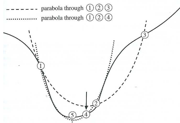
FIGURE 2.11 – Brent's method in one dimension to find a minimum with parabola interpolation : source [Press et al., 2007]
