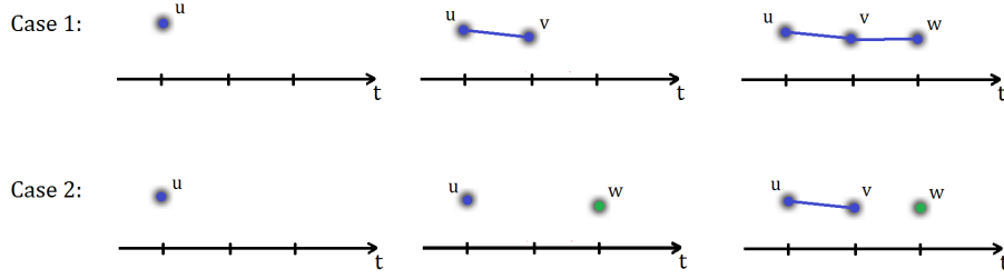
Figure 5.10: The state of the Markov chain depends on the order in which the objects are added to the configuration. Case 1: \mathbf{X} = ((\mathbf{X} \cup u) \cup v) \cup w (first u , then v and then w was created). Case 2: \mathbf{X} = ((\mathbf{X} \cup u) \cup w) \cup v (first u , then w and then v was created).
