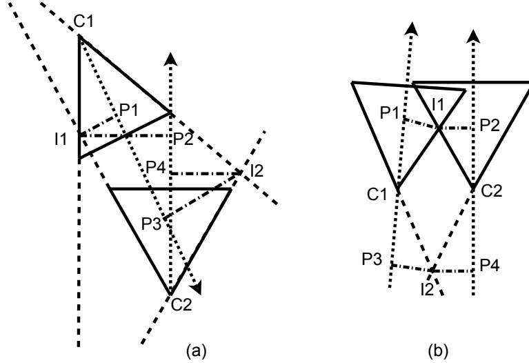
Figure 3.8: Frustum collision test; the continuous lines indicate the frustum and the dotted arrows indicate the forward vectors.
