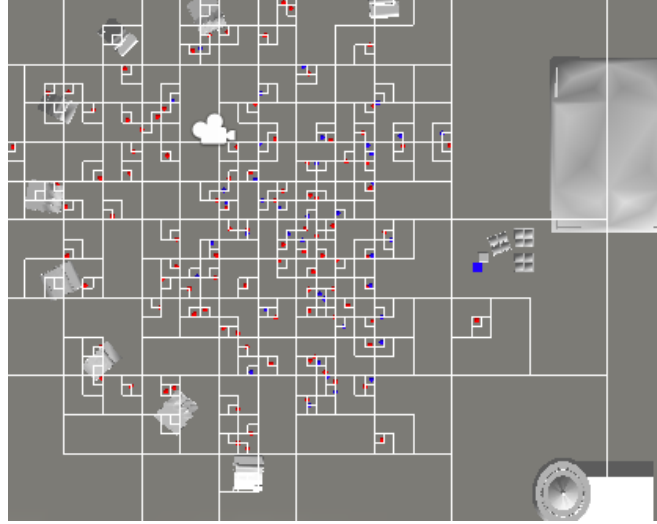
Figure 3.10: Using a quad-tree representation to reduce computational cost in querying characters in camera frustums and detecting events.
