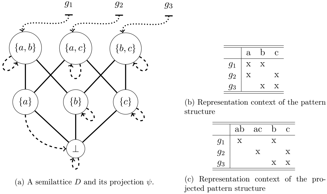
Figure 5.4: An example of a projection that can increase the number of attributes in the minimal representation context.
