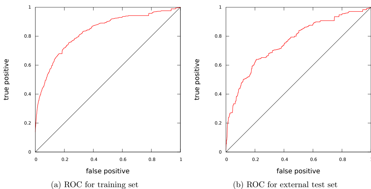
Figure 4.4: ROC plots for the training set (left) and the external validation set (right).
