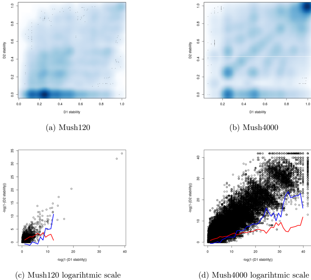
Figure 2.2: Stability in the test dataset w.r.t the reference one.
