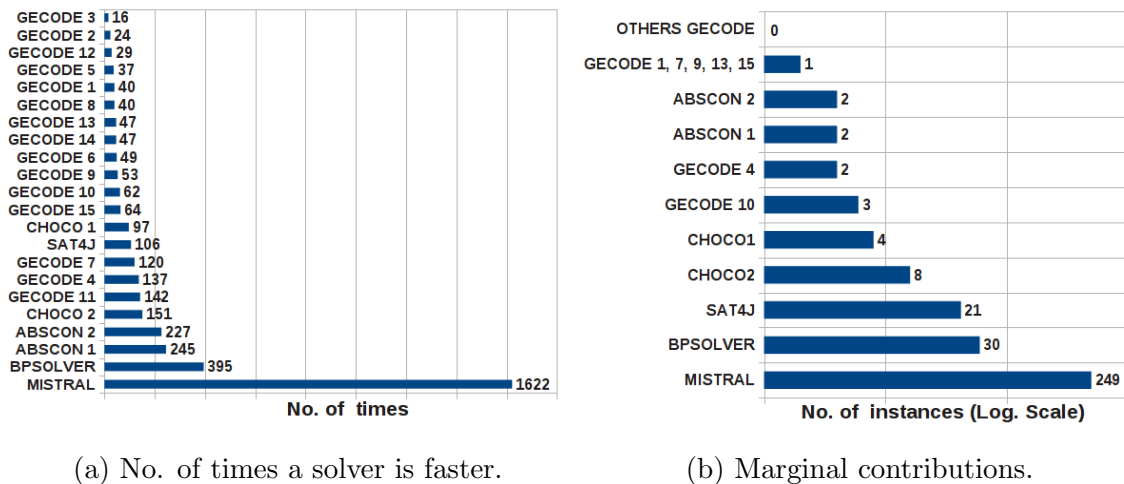
Figure 4.1: Solvers statistics.
