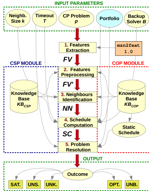
Figure 6.1: sunny-cp architecture.
