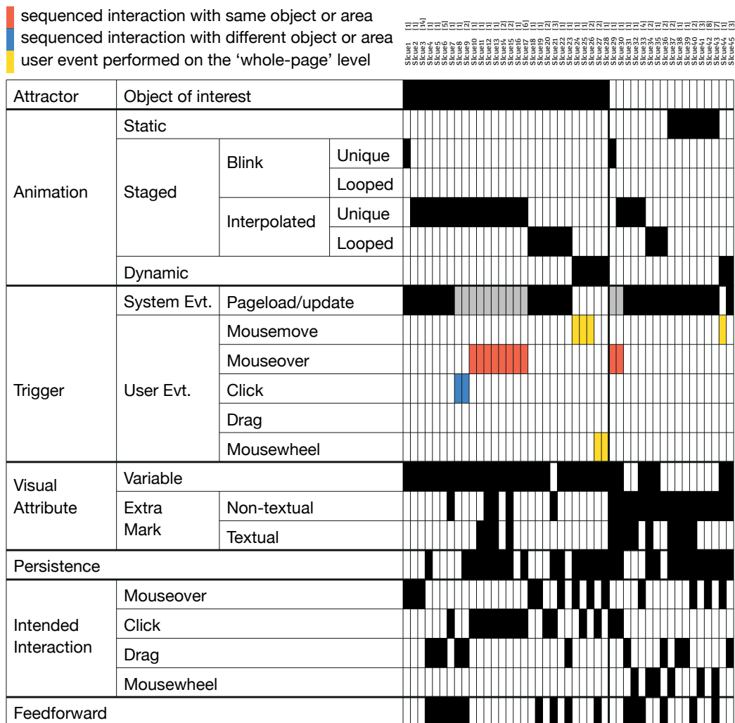
FIGURE 5.6: A design space of SI, based on our survey of 382 HTML5 and visualization websites. Due to space limitations, the table has been transposed, so entries are columns and dimensions are rows. The count of occurrences of each SI cue is shown in brackets, and the cue names refer to minified URLs (e.g., SIcue1 can be retried at http://tiny.cc/SIcue1 ). Note that several URLs direct to the same websites, as these include multiple distinct SI cues. Finally, an interactive version of the design space with animated GIFs of each cue is available at [9].
