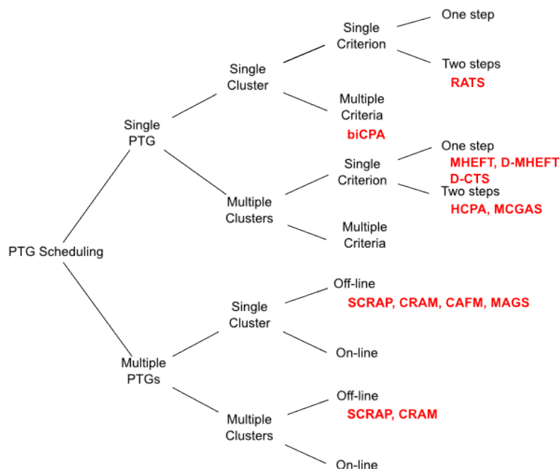
Figure 1.22: A taxonomy of Parallel Task Graph scheduling problems with the proposed heuristics.
