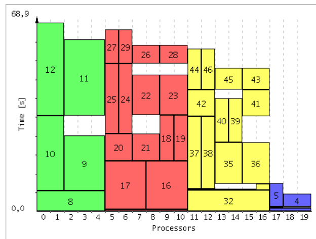
Figure 2.14: Jedge output for the schedule produced by one of the algorithms proposed in [CDS10]. Four PTGs, each having its own color, are scheduled on a cluster of 20 processors. The resource constraints imposed by the algorithm are respected.
