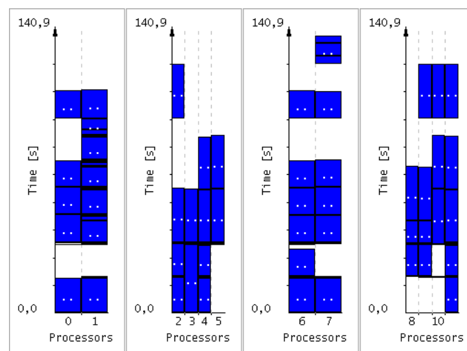
Figure 2.15: Jedge output of the schedule by HEFT of a DAG of 50 task on a heterogeneous platform.
