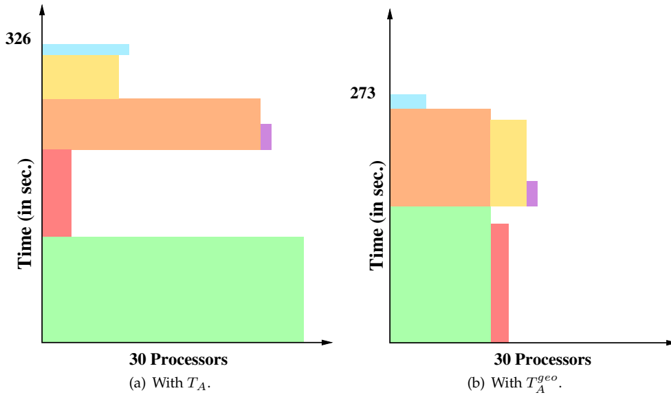
Figure 1.8: Gantt chart of the schedule of a six-task PTG on a cluster of 30 processors using the original T_A (a) and T_A^{geo} (b).
