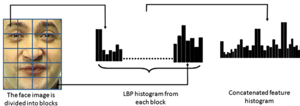
Figure 7: LBP Histogram computation [2]
