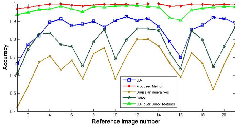
Figure 39: Recognition rate with different reference images
