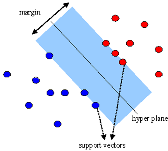
Figure 8: SVM classifying linearly separable data [5]
