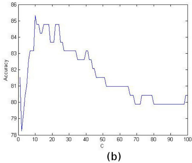
Figure 31: (a) Graph of classification accuracy vs. C-parameter and 1/\gamma for pleasure and (b) Graph of accuracy vs. C-parameter at 1/\gamma = 190 for pleasure
