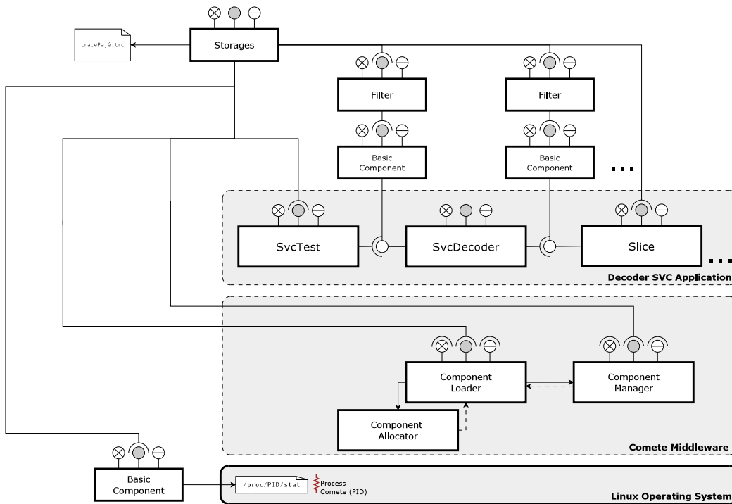
Figure 2.5 – Partial representation of the EMBera Observation Components in the SVC use case [190]
