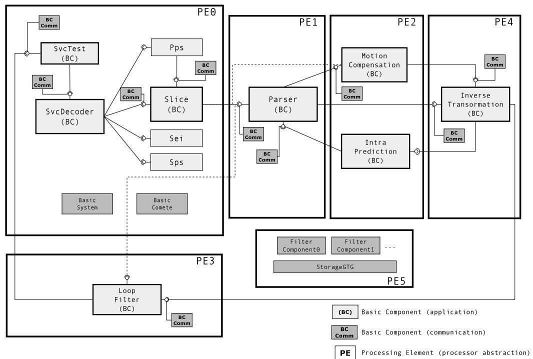
Figure 2.4 – EMBera Components in the SVC Application [190]
