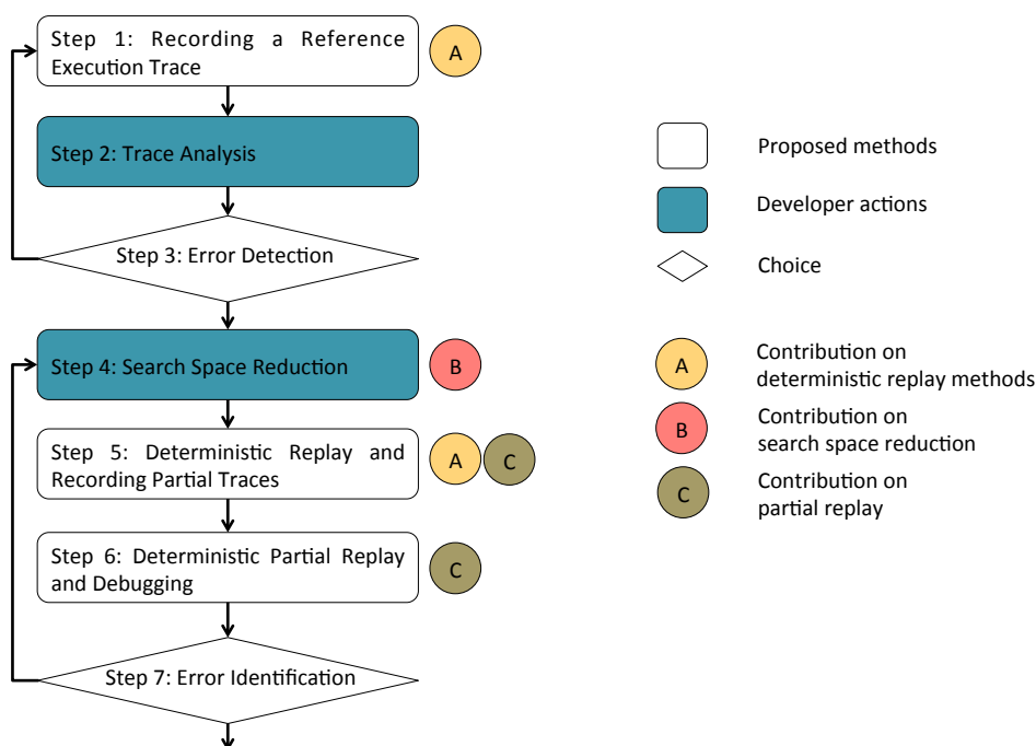
Figure 3.2 – Debugging Cycle
