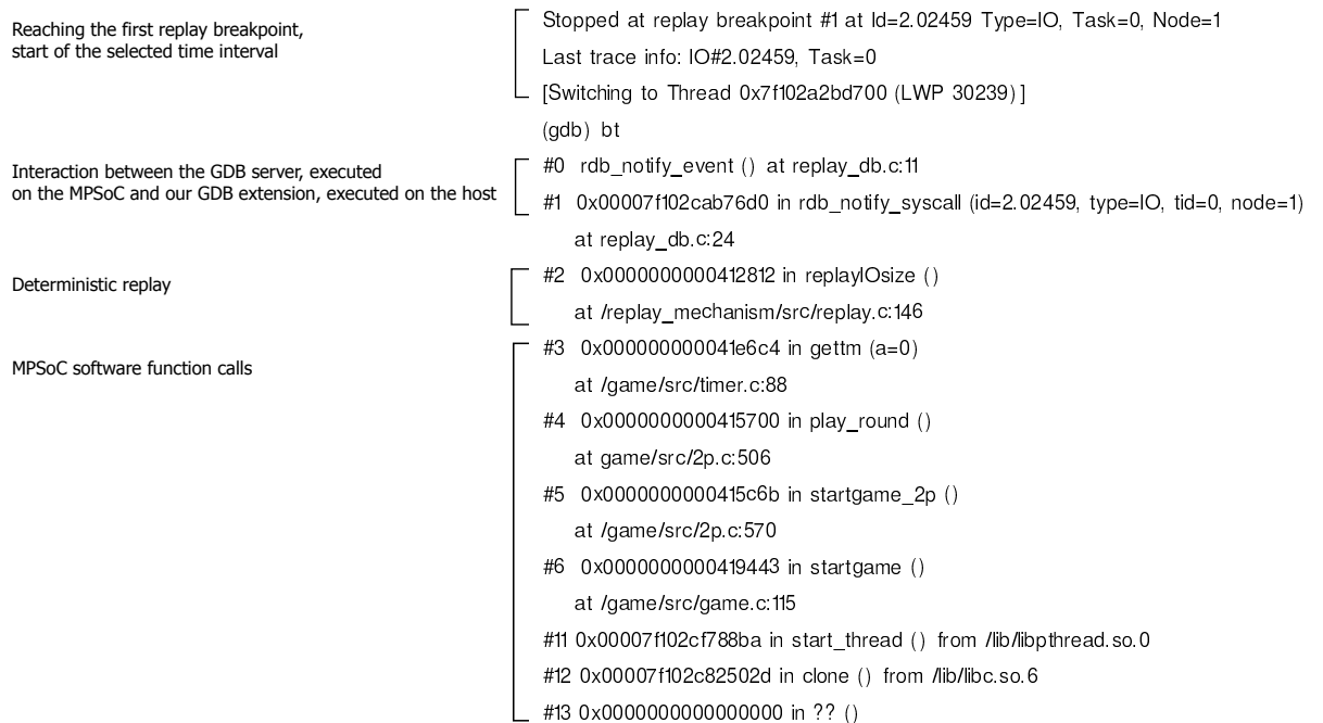
Figure 3.5 – Partial Debugging of the MPSoC Tetris Application
