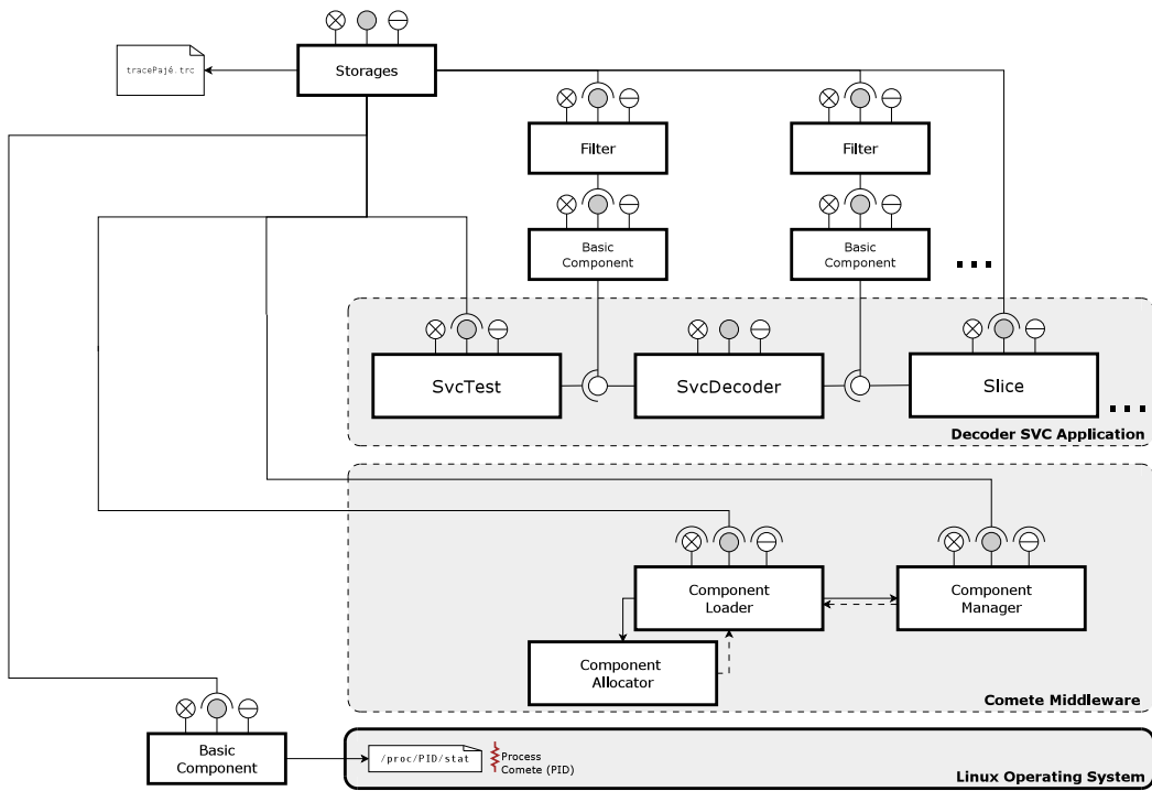
Figure 2.5 – Partial representation of the EMBera Observation Components in the SVC use case [190]
