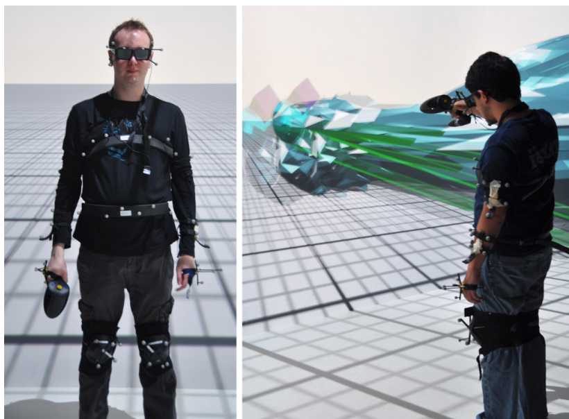
Figure 3.13 – Setup of our experiment. A subject with 11 position trackers used to record his posture and a Flystick to manipulate the objects (left), and a manipulation scenario of the 7-Handle technique in an immersive virtual environment (right).
