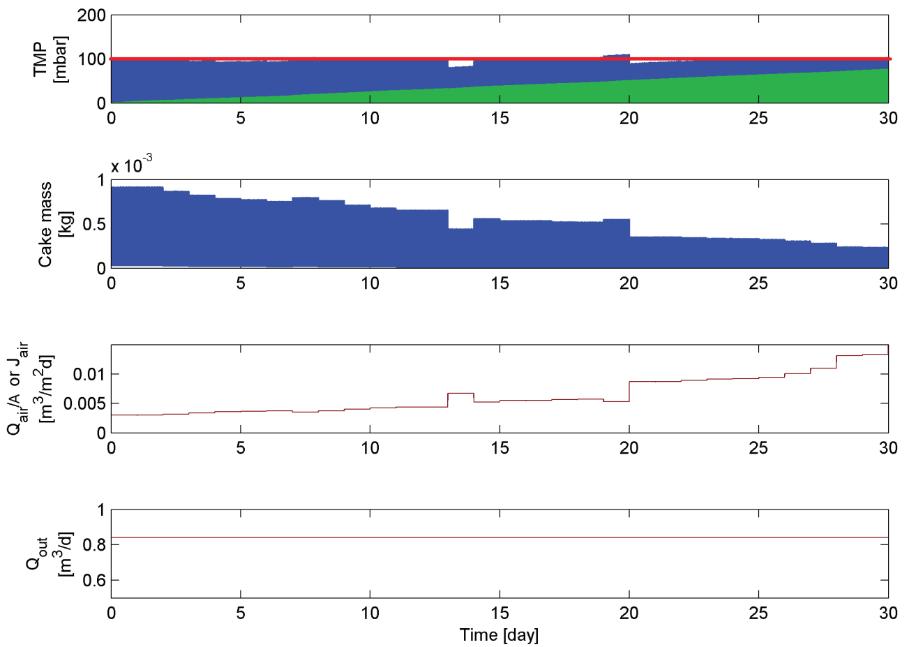
Figure 5.2: The NMPC acting on the descriptive process.
