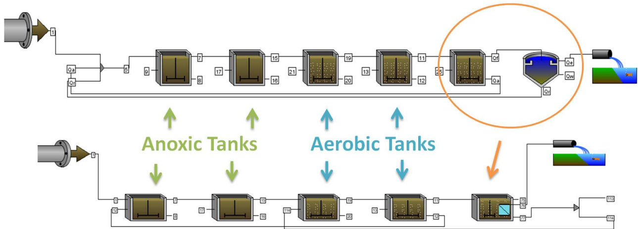
Figure 1.7: Conventional Activated Sludge versus sMBR.
