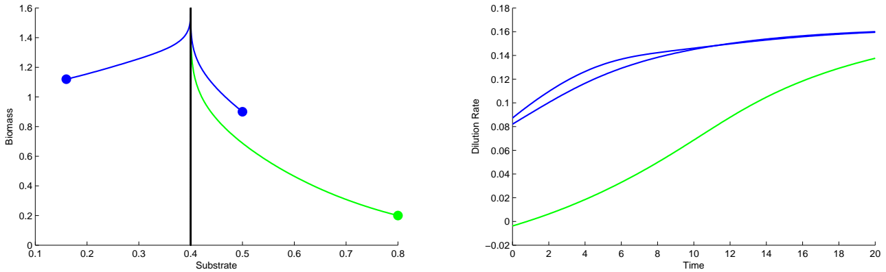
Figure A.3: Quadratic Lyapunov Functions with \lambda_1 = 1 .
