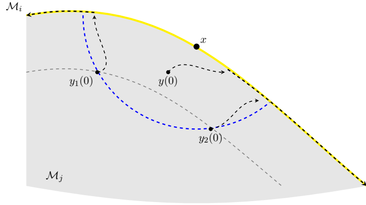
Figure 7.4: Illustration of Lemma 7.4.1
