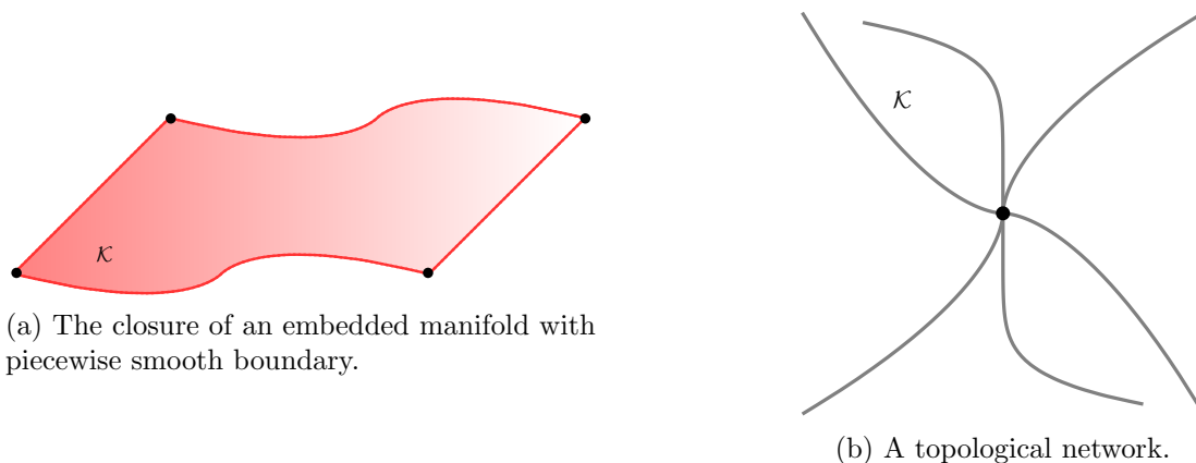
Figure 1.3: Some further examples of stratifiable state-constraints sets.
