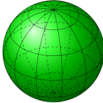
Figure 3.1: The sphere of radius 1.
