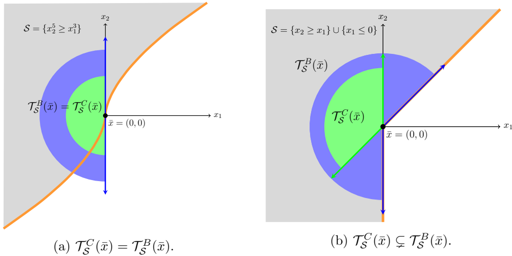
Figure 2.1: Some examples of tangent cones.
