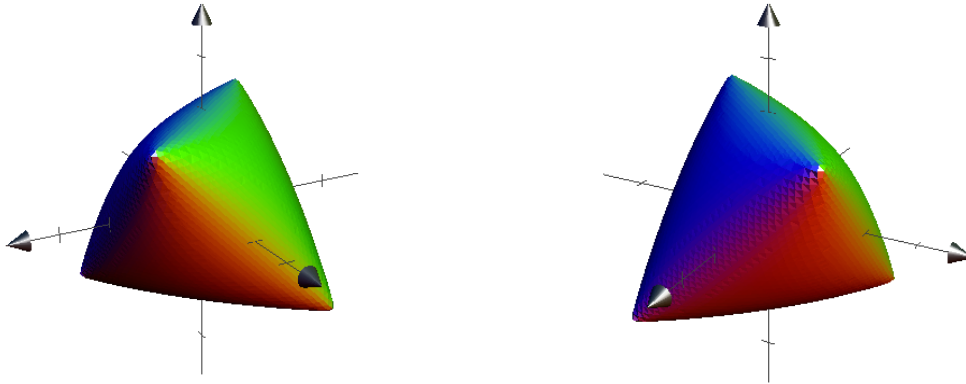
Figure 3.5: Different angles of the semialgebraic set of Example 3.3.1.
