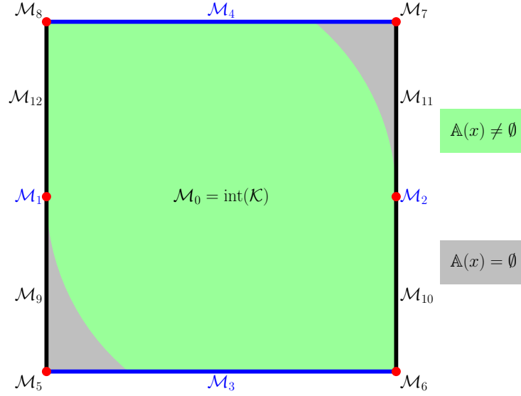
Figure 4.4: The stratification of Example 4.2.1.
