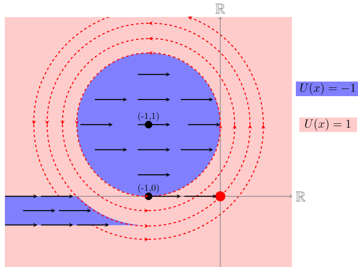
Figure 1.7: An Illustration of Example 1.2.4.
