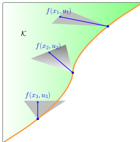
Figure 1.1: An example of Inward Pointing Condition.
