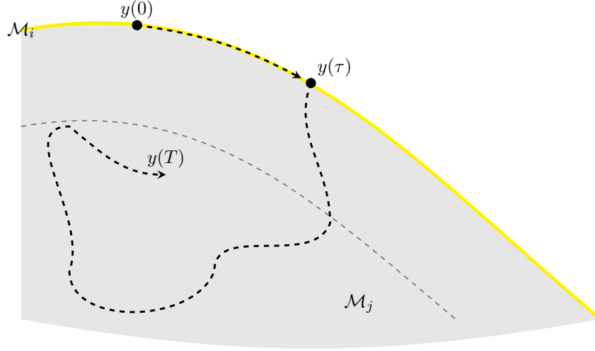
Figure 7.6: Illustration of Lemma 7.4.2
