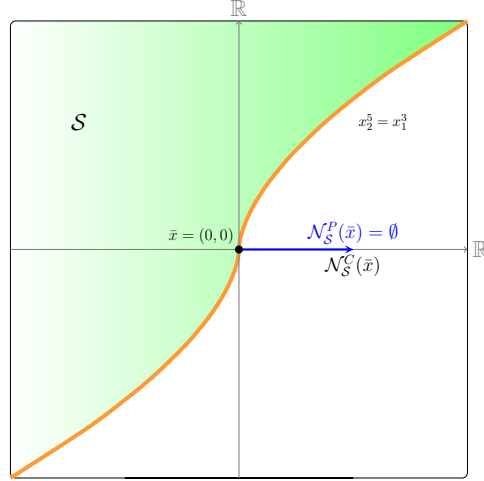
Figure 3.2: The set \mathcal{S} in Example 2.3.2.
