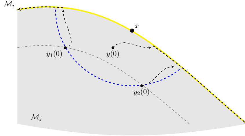
Figure 7.4: Illustration of Lemma 7.4.1
