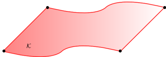
(a) The closure of an embedded manifold with piecewise smooth boundary.
