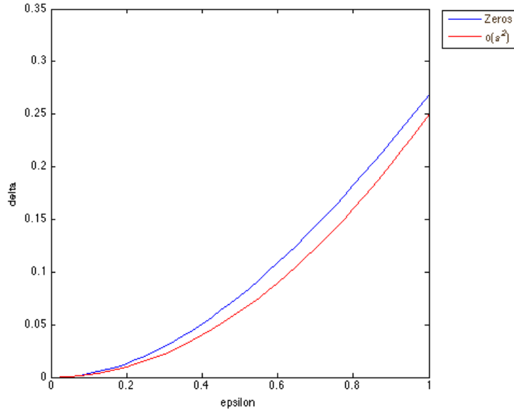
Figure 8.6: The zeros of the \chi_\varepsilon .
