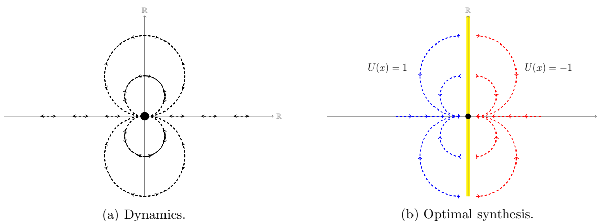
Figure 1.5: The Artstein's Circles.
