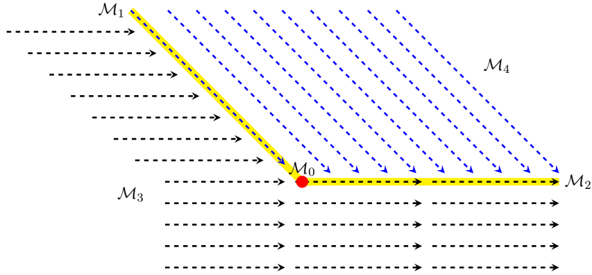
Figure 7.5: Example Remark 7.4.3
