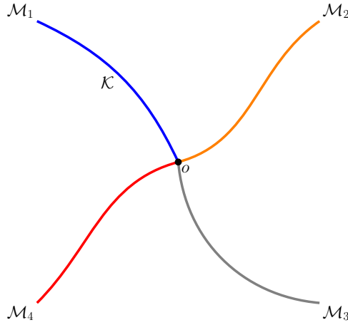
Figure 9.2: An example of a network in \mathbb{R}^2 .
