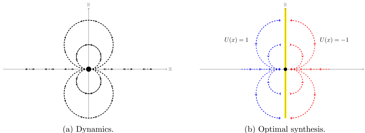
Figure 7.1: The Artstein's Circles.
