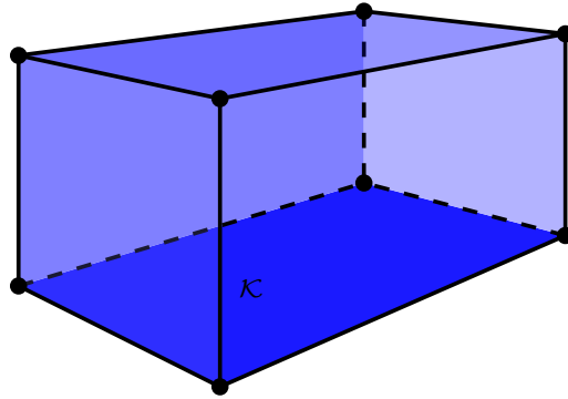
Figure 3.4: A semilinear set in \mathbb{R}^3 .
