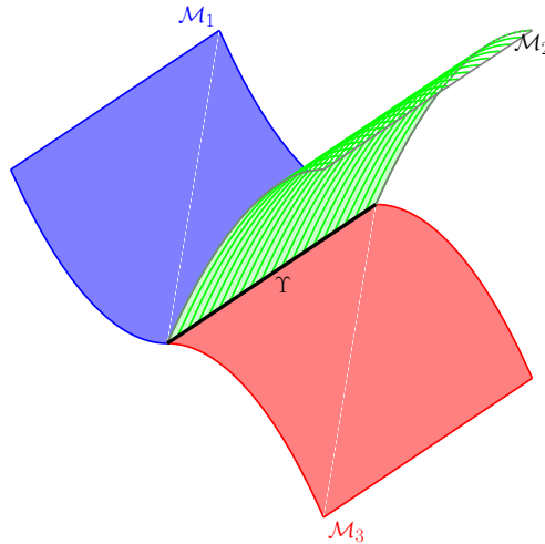
Figure 9.5: A 2-dimensional junction embedded in \mathbb{R}^3 .
