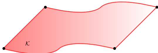
(a) The closure of an embedded manifold with piecewise smooth boundary.
