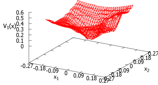
Figure 4.7: CPA ISS Lyapunov function in dissipative formulation V_1 delivered by the algorithm for system (4.76) with the gain parameter r = 2.89335 .
