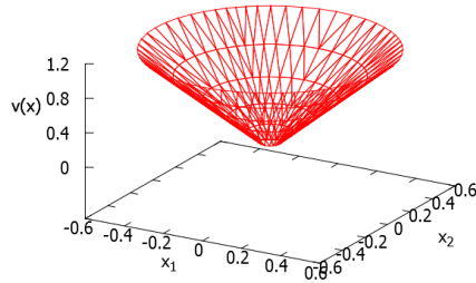
Figure 4.2: Theoretical CPA ISS Lyapunov function in dissipative formulation v based on the function W_2 for system (4.57), \epsilon = 0.048 , r_2 = 0.4410 .
