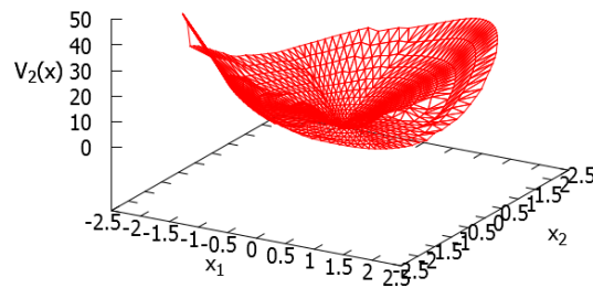
Figure 4.6: CPA ISS Lyapunov function in dissipative formulation V_2 given by the algorithm for system (4.63), \epsilon = 0.012 , r = 19.7621 .
