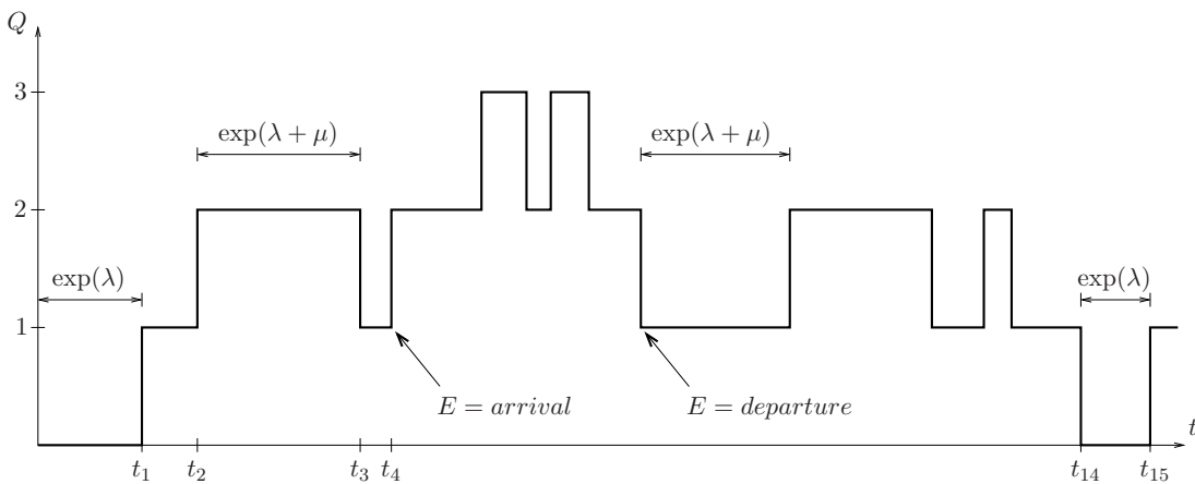
Figure 5.6: A trial of an M/M/1 Queueing System
