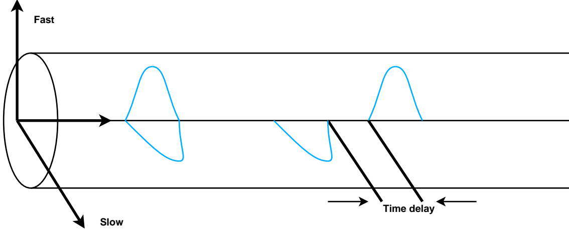
Figure 7.4: Delay in optical fiber.
