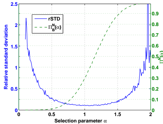
Figure 7.3: Proportion of particle above B at final time and relative standard deviation.
