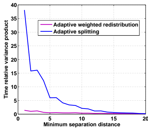
(b) Time relative variance product.
