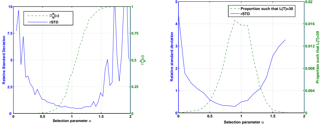
(a) Proportion of particles above B at final time and (b) Proportion of particles such that L(T) = 30 at final time and relative standard deviation.
