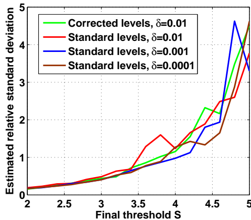
Figure 5.6: Estimation of the relative standard deviation in the estimation of (5.14) with the corrected and standard regions.
