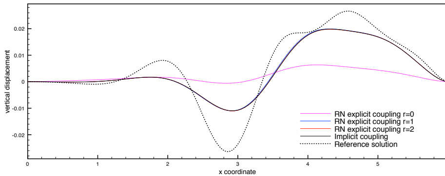
Figure 3.3: Interface vertical displacement at time t = 1.5 \cdot 10^{-2} , with \tau = 2 \cdot 10^{-5} and h = 0.05 , (undamped solid).
