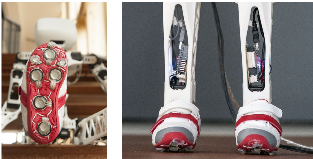
Fig. 8.16.: Physical implementation of the sensors on Poppy. FSR have been placed under feet while Arduino nano board are placed on the leg acquire the data and stream them to the main IO board through USB.
