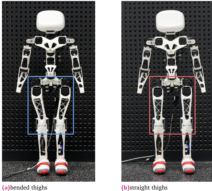
Fig. 8.1.: We evaluate the effect of thigh morphology on the bipedal locomotion dynamic. Experiments are made using the Poppy humanoid platform. In this paper, we compare two thigh morphologies: (a) thigh bended by an angle of 6^\circ and (b) a more classical approach with straight thighs.
