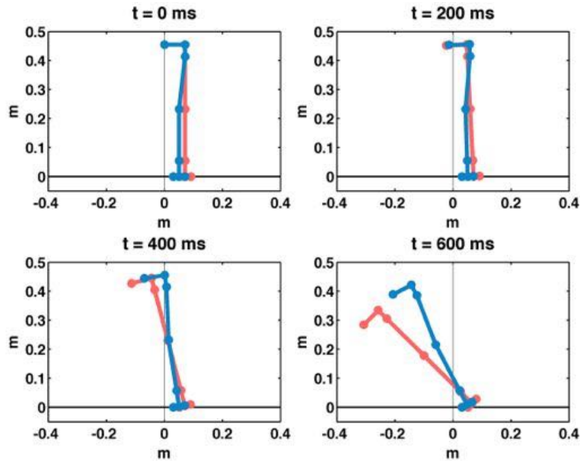
Fig. A.2.: Comparison of the falling dynamic over time when Poppy is standing on one foot, depending on its thigh morphology: with a bended thigh of 6^\circ (blue) and with a straight thigh (red).
