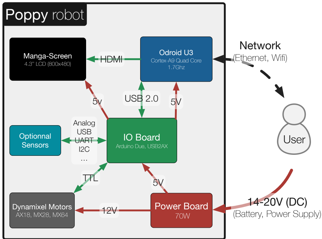
Fig. 6.16.: Overview of the Poppy electronics architecture.
