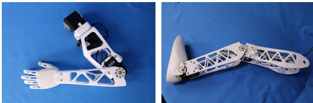
(a) Poppy's arm mechanical structure
