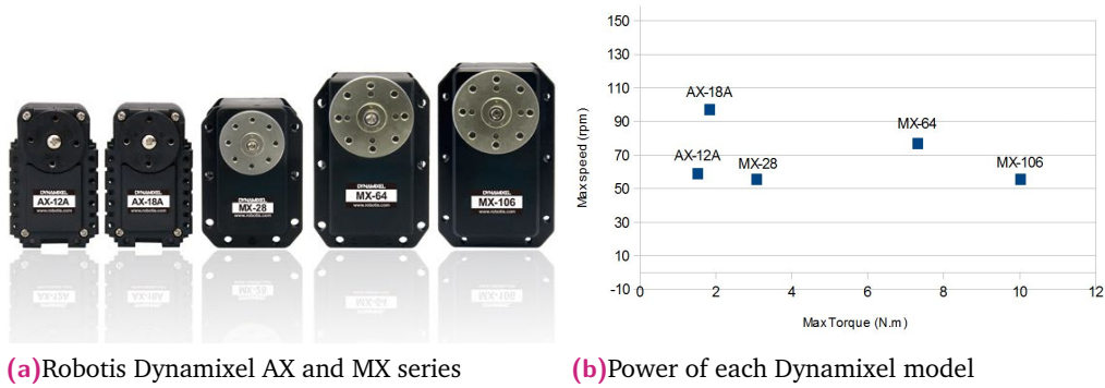
Fig. 5.4.: The Robotis Dynamixel come with different models from low-cost ones such as AX-12/18 to the most powerful MX-series with Maxon motor and magnetic encoder.
