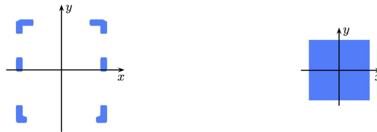
Fig. 6.7.: Comparison of poppy's leg section and a rectangular beam having the same second moment of area.
