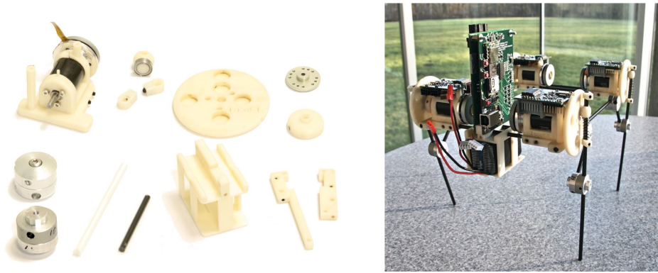
Fig. 3.2.: The Locokit is a multi-purpose hardware kit to study several morphological properties.
