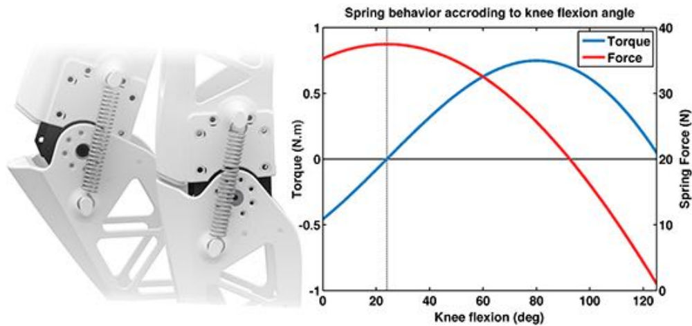
Fig. B.2.: Theoretical semi-passive mechanism behavior. The blue line corresponds to the torque applied by the springs on the leg according to the flexion angle of the knee. The red line corresponds to the force that the springs applied on ties.
