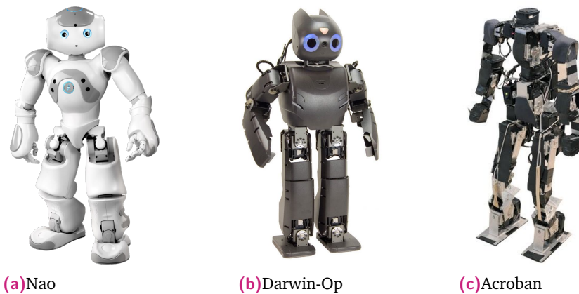
Fig. 6.1.: None of the existing platforms in 2012 was suitable for exploring the role of morphology. Nao was impossible to modify. Darwin Op and Acroban used aluminium parts that are really difficult and expensive to produce.
