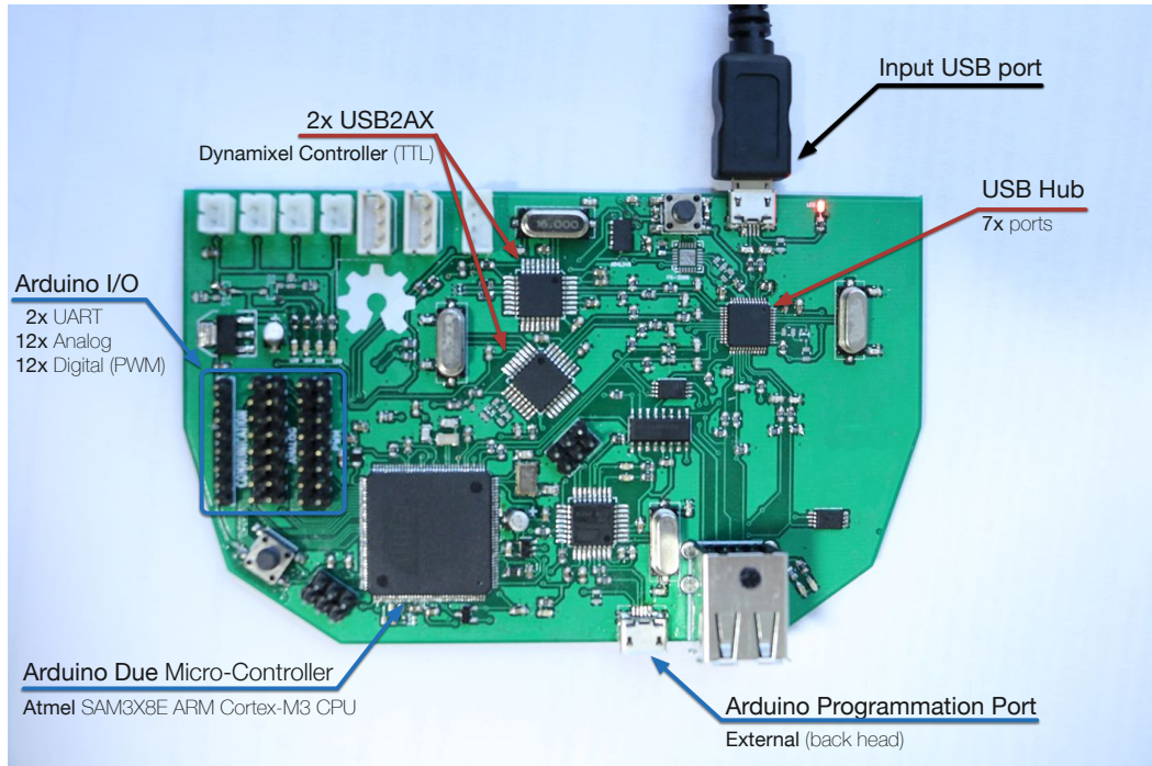
(a) Current design of the IO Board.
