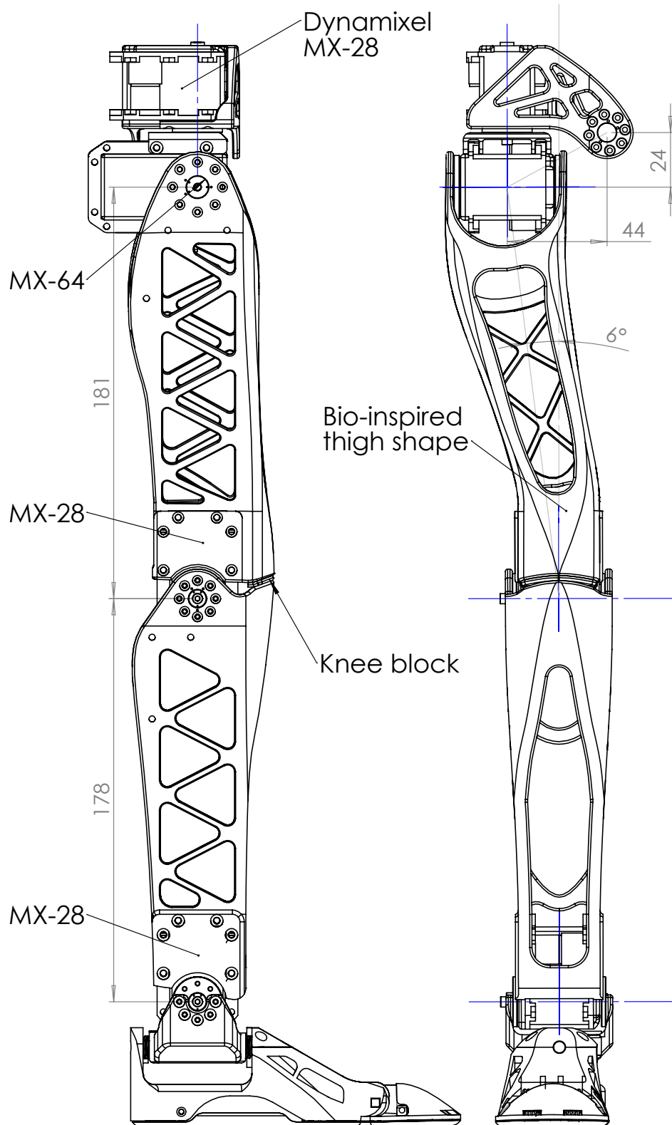
Fig. 6.11.: Blueprint of Poppy's right leg. Parts have a truss structure to reduce the mass, and each leg has 6 DoF. Only the one on the hip use powerful motors (MX-64), others are powered by MX-28. This choice makes the robot could not support its weight if knees keep bended during walking. Therefore it constraints the research of more human-like gait with straight support leg.
