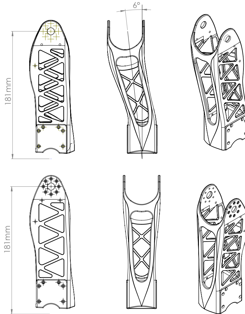
Fig. 8.3.: Blueprints of the two thighs tested in this experiment. The only parameter explored is the bending angle of the thigh: 6^\circ and 0^\circ
