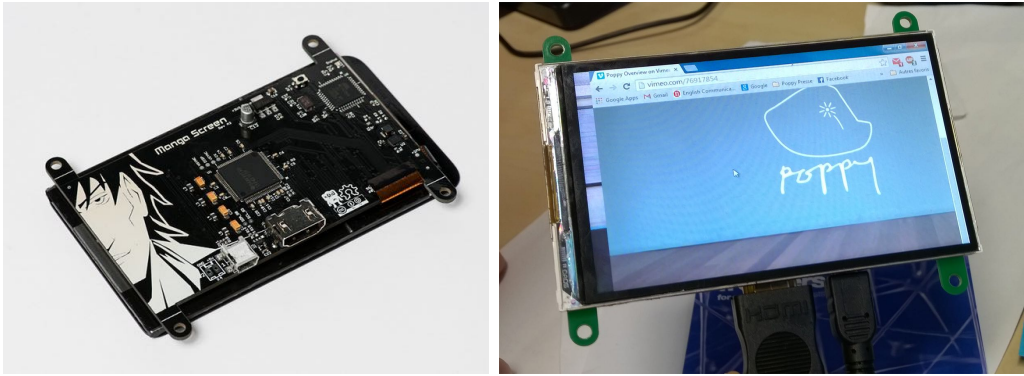
Fig. 6.20.: The future face display embedded in Poppy is an open source project called manga-screen (see https://bitbucket.org/intelligentagent/manga-screen/ ). This project is the only one we have found allowing to have both a 4.3inch display and HDMI connexion.
