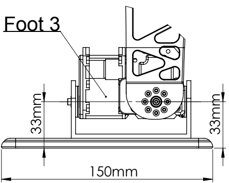
(e)Blueprints of the various foot designs studied in this experiments.
