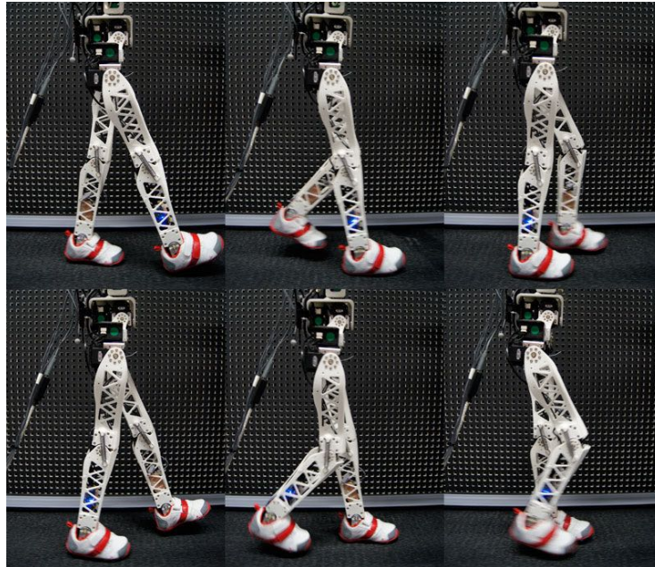
Fig. 8.8.: Walking gait CPG described on Fig. 8.7.d applied on the actual Poppy robot. The CPG generates a human-like walking gait allowing the robot to walk at 1.8km/h and involves straight legs during the stance phase. There is no balance control, but stability is obtained through physical guidance with a trained expert user.
