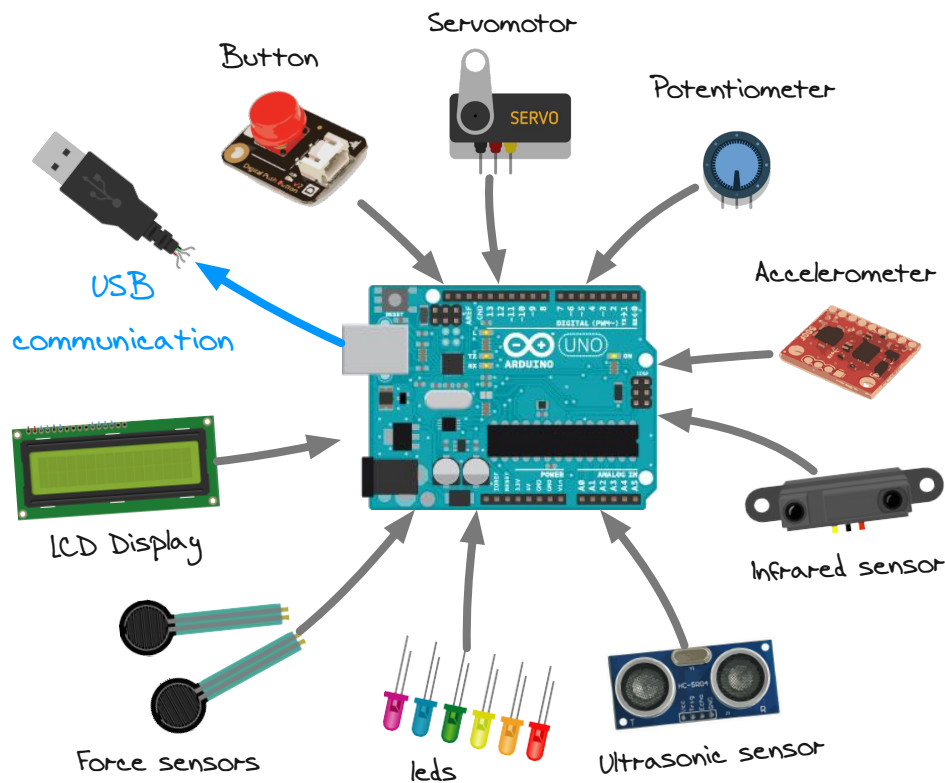
Fig. 5.3.: The use of Arduino as electronic architecture allows for sensors to be easily added and/or changed while keeping the same electronic board. In addition, it permits to add expressive components such as LEDs, LCD or sound systems, allowing users to easily explore human-robot interaction.
