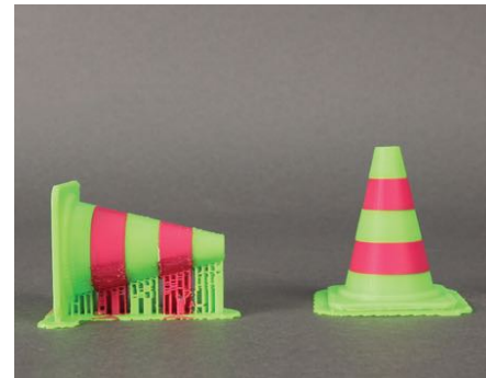
(b) FDM result example
