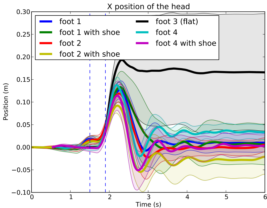
Fig. 8.13.: Evolution of the position of the head in the x axis for each foot tested (see Fig. 8.11 for illustration of each foot)
