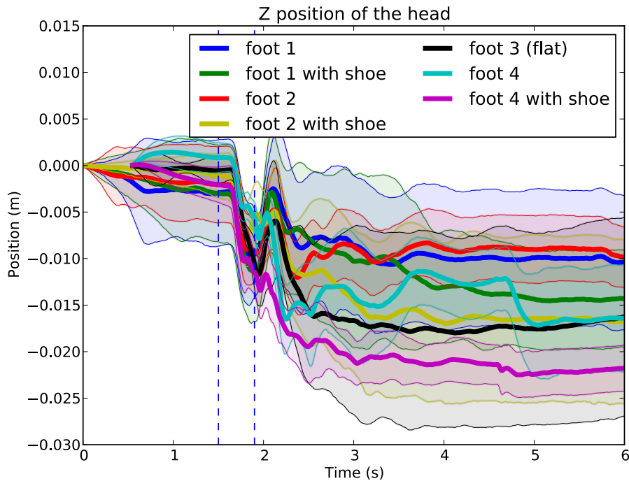
Fig. 8.15.: Evolution of the position of the head in the z axis for each foot tested (see Fig. 8.11 for illustration of each foot).
