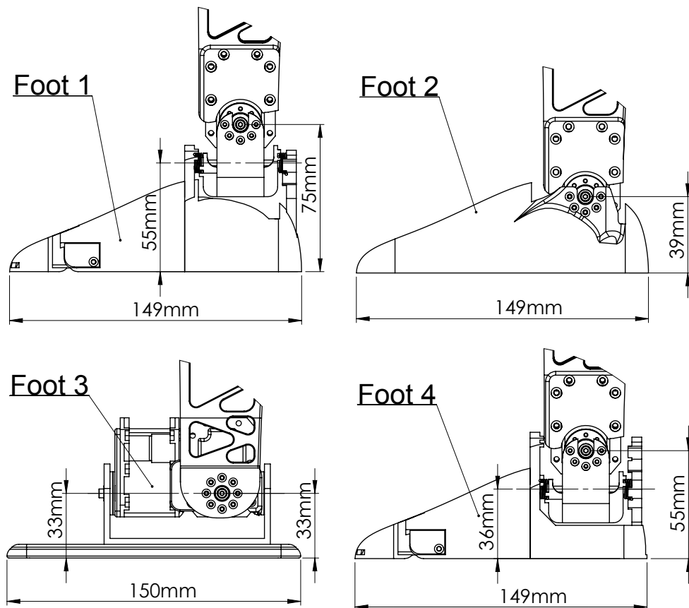
(e)Blueprints of the various foot designs studied in this experiments.
