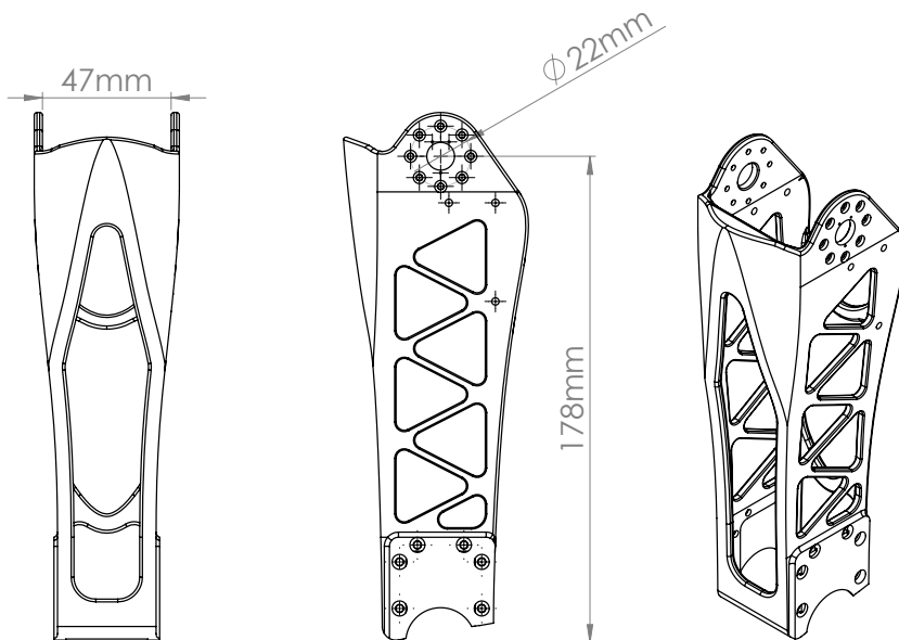
Fig. 6.4.: Example of the use of mechanical configuration. Here the CAD source of the leg involves 2 configurations so it can be compatible with Dynamixel MX-28 (up) or Dynamixel MX-64 (down). Configuration defines the set of parameter suitable for both and can be changed just in one mouse click.
