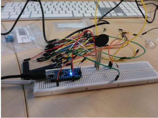
(a) A FSR sensor connected with Arduino nano board.
