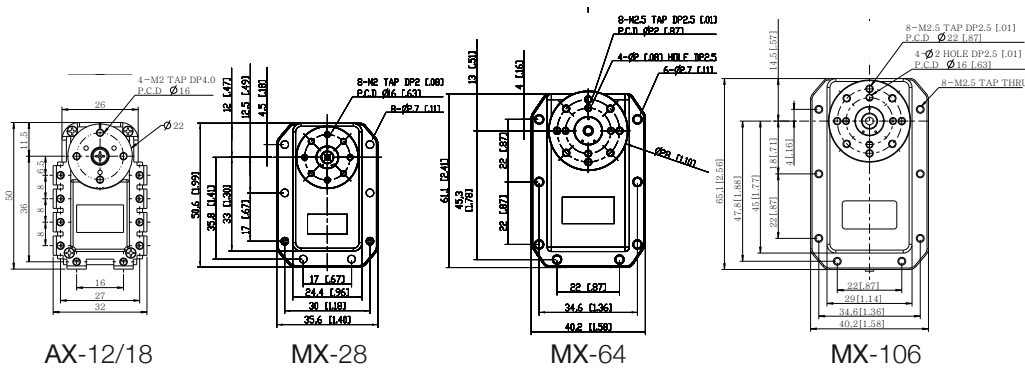
Fig. 5.5.: The footprint of Dynamixel motors keeps the same pattern, only the dimensions are increased following the power of the motor. Thus, switching from one model to another only requires changing the dimension and not the design of a part. With parametric CAD software such as Solidworks, it takes a couple of minutes to modify a mechanical part to be compatible with another Dynamixel motor.
