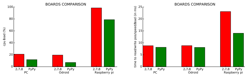
(b) CPU load when pypot run on Poppy to synchro- (c) Time spent in each synchronization loop for 25 nize the 25 motors motors
