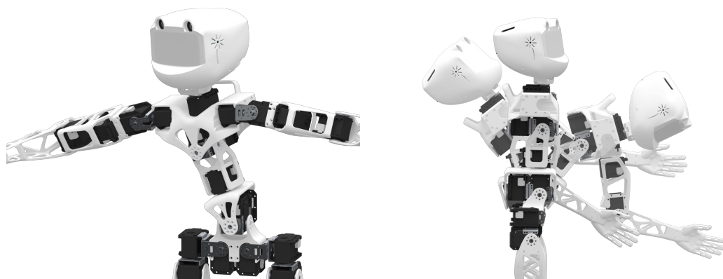
Fig. 6.14.: This figure shows the blueprint of Poppy's 5 DoF torso as well as illustration of the resulting mobility.
