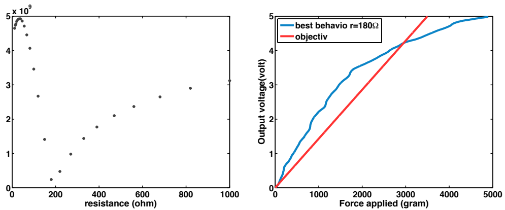
(a) Optimization of the voltage divider constant resistor: distance between the output behavior with respect to a linear behavior. (b) Theoretical behavior (blue) of the output voltage with respect to the applied force with a 14v input and a 180\Omega compared with the objective linear behavior.
