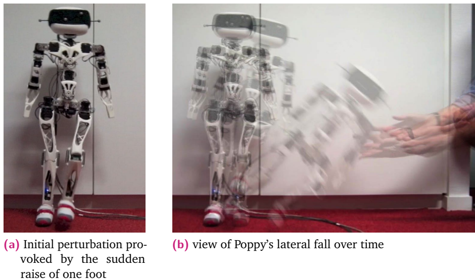
Fig. 8.4.: Run of the single support falling experiment. The markers on Poppy's headband track its absolute position over time.
