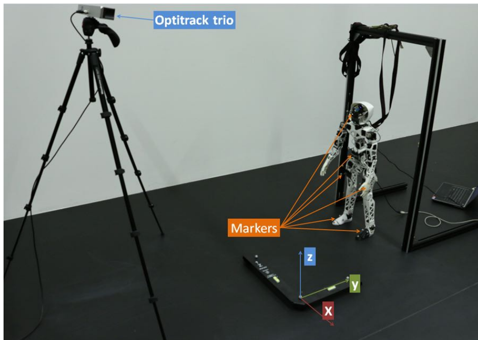
Fig. 8.12.: Experimental setup. The robot is secured by slack strap on a gantry and tracked by an OptiTrack trio device. Markers are placed on the feet, hips, abdomen, and on the head
