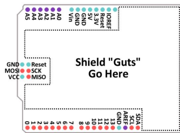
(a) Arduino form factor
