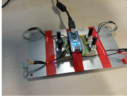
(b) Simple testing assembly with 4 voltage dividers with FSR sensors and potentiometers plugged on an Arduino nano board
