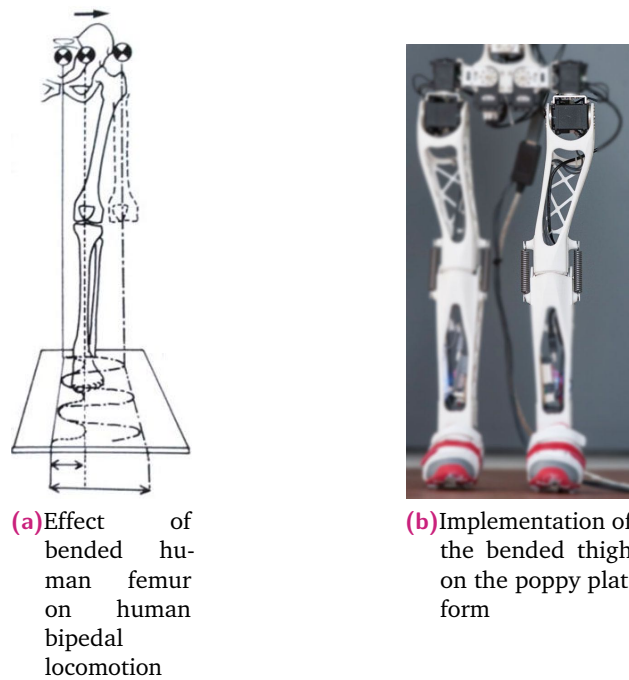
Fig. 8.2.: The human femur is inclined by an angle of 6^\circ , this reduces the distance traveled by the CoG to be supported from one leg to the other during walking. We reproduced it on Poppy and suggest exploring its impact on the robot dynamics.
