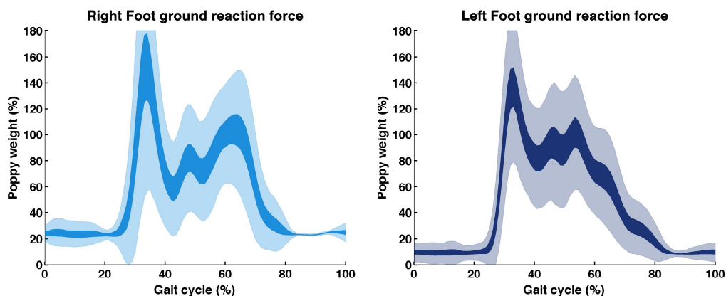
Fig. 8.17.: Ground reaction forces measured with the FSR sensors placed under Poppy's feet.
