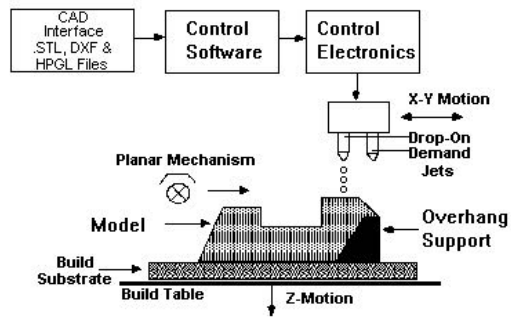
(a) FDM process
