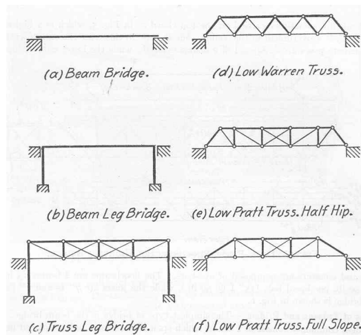
Fig. 6.6.: The truss structure has been massively used in civil engineering, especially to construct bridges. Here is shown several truss structure configurations.
