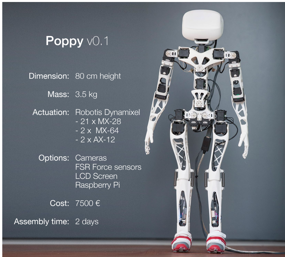
Fig. 6.2.: Overview of Poppy beta with the main specs and features. This figure will be updated when the final release of Poppy is ready.
