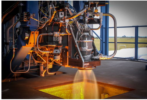
(a) The SuperDraco rocket engine has a combustion chamber: 3D-printed - SpaceX.
