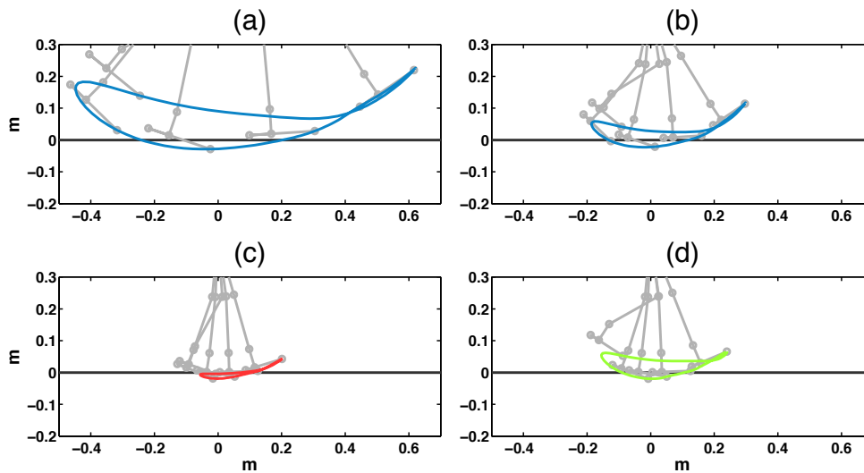
Fig. 8.7.: Trajectories of toes generated by the walking pattern a) Kinematics of human walking with human morphology b) Direct transposition of human kinematics onto Poppy's morphology c) Reducing amplitude of the human kinematics joints with Poppy's morphology d) Walking pattern used for the experiment with Poppy
