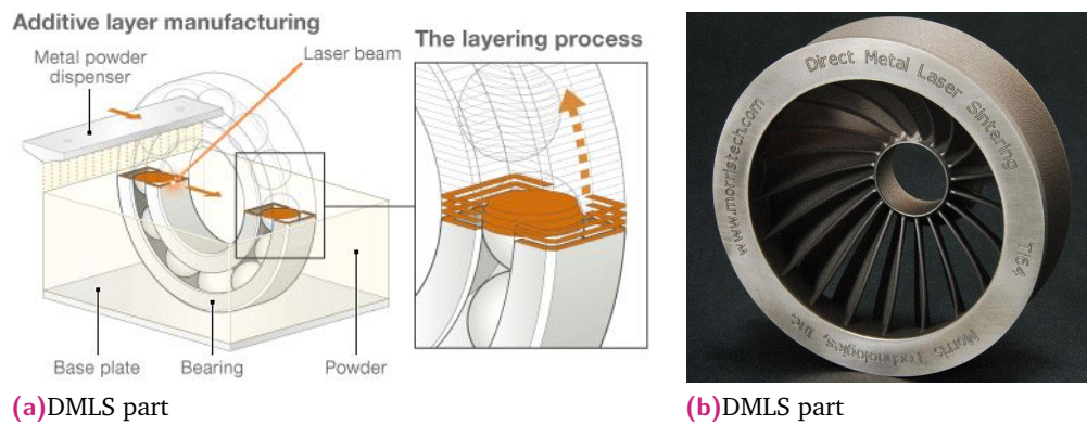
Fig. 4.5.: Direct Metal Laser Sintering is very similar to the SLS process but uses a high-powered 200 watt Yb-fiber optic laser in order to fuse metal powder into a solid part by melting it locally.
