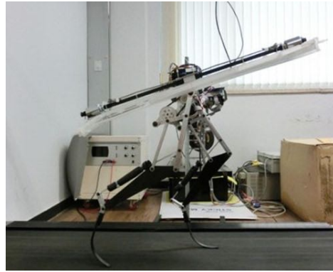
(b) Raptor has both compliant actuators and feet. It is currently the fastest bipedal robot.
