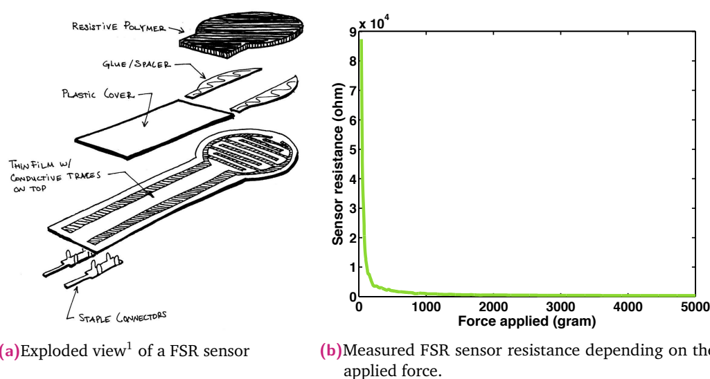
Fig. C.1.: The FSR force sensors are cheap, but they have a really non-linear behavior and are not very precise.
