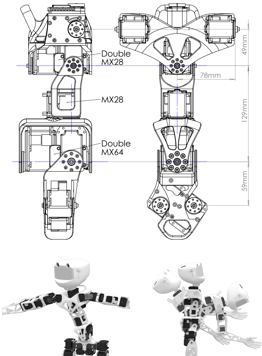
Fig. 6.14.: This figure shows the blueprint of Poppy's 5 DoF torso as well as illustration of the resulting mobility.
