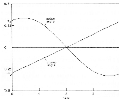
(b) The stance leg rolls forward steadily like a spoke in a wheel while the free leg swings ahead like a pendulum. Support is transferred between legs when their speeds and angles match.
