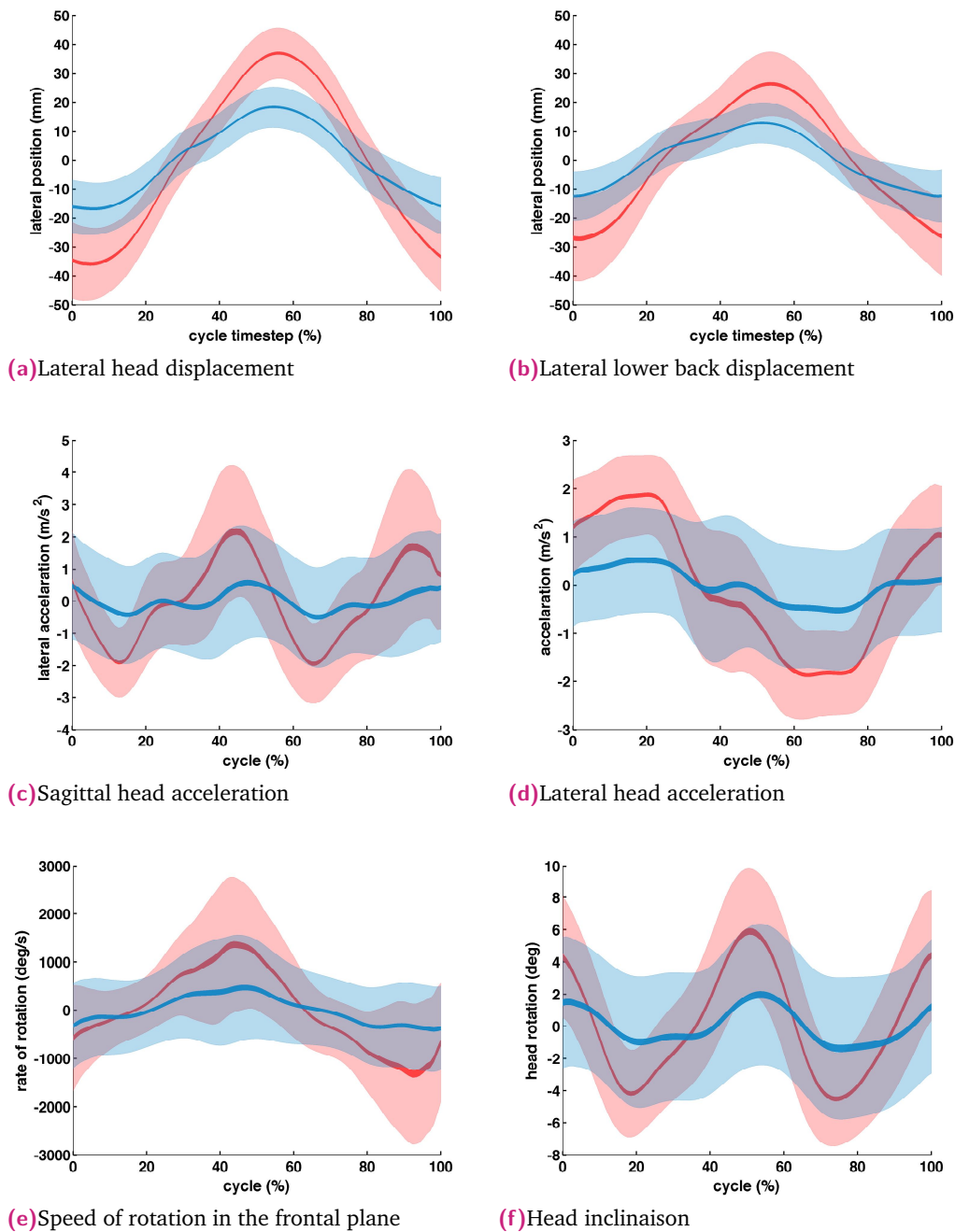
Fig. 8.9.: Results obtained during the walking experiment. The blue color is associated with experiments conducted with bended thighs while the red color is assigned to straight thighs. For each case, the light color corresponds to the standard deviation and the dark color to the 95% confidence interval of the mean value. All data are folded over to extract the mean gait behavior and its standard deviation over a walking gait cycle expressed in percent.
