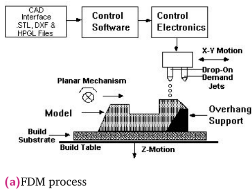
Fig. 4.2.: The FDM technique relies on melting and selectively depositing a thin filament of thermoplastic polymer (ABS - PLA) in a cross-hatching fashion to form each layer of the part.
