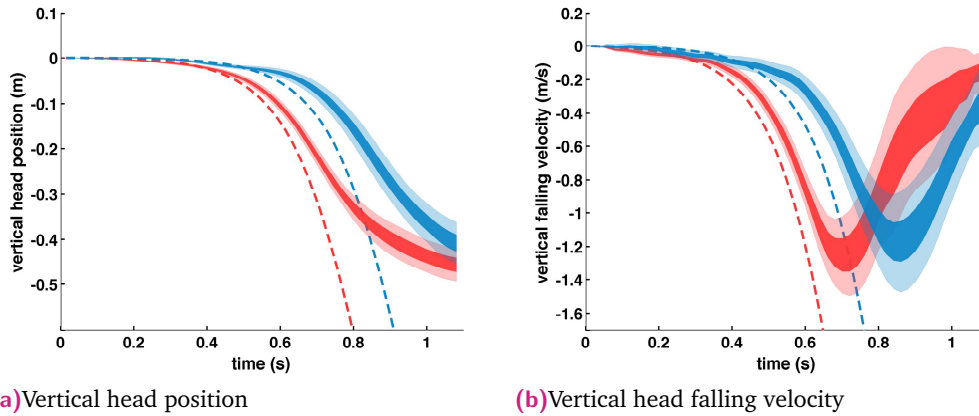
Fig. 8.5.: Results of the single support falling experiment. The blue color is associated with experiments conducted with bended thighs while the red color is assigned to straight thighs. For each case, the light color corresponds to the standard deviation and the dark color to the 95% confidence interval of the mean value while dashed lines represent theoretical results. These figures show the vertical position (a) and vertical falling velocity (b) of the head of Poppy over time for each case studied. The curve's behavior change after 800 min is due to the fact that we catch the robot before it touches the ground.
