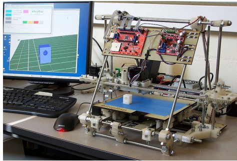
(a) RepRap v2
