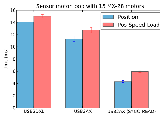
(c) Comparison of communication speed. We can notice the strong speed improvement the SYNC_READ instruction brings to the USB2AXS
