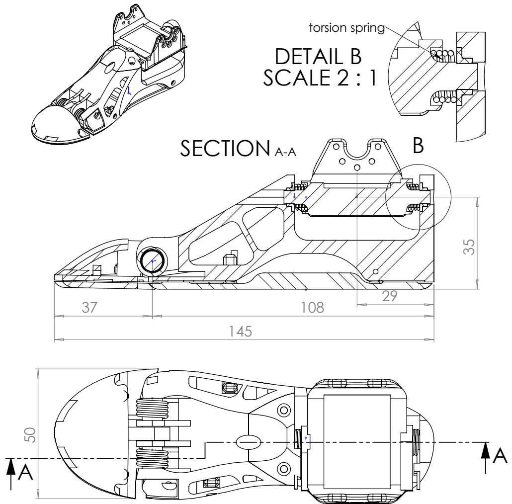
Fig. 6.10.: Blueprint of Poppy's foot. This foot has two passive joints, one for the toes, and one for the ankle roll. As we can see on the section A-A and detail B, both use torsion springs.
