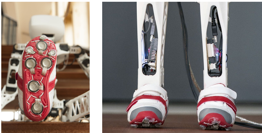
Fig. 8.16.: Physical implementation of the sensors on Poppy. FSR have been placed under feet while Arduino nano board are placed on the leg acquire the data and stream them to the main IO board through USB.
