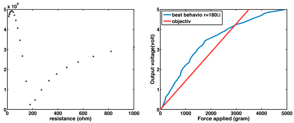
(a) Optimization of the voltage divider constant resistor: distance between the output behavior with respect to a linear behavior. (b) Theoretical behavior (blue) of the output voltage with respect to the applied force with a 14v input and a 180Ω compared with the objective linear behavior.
