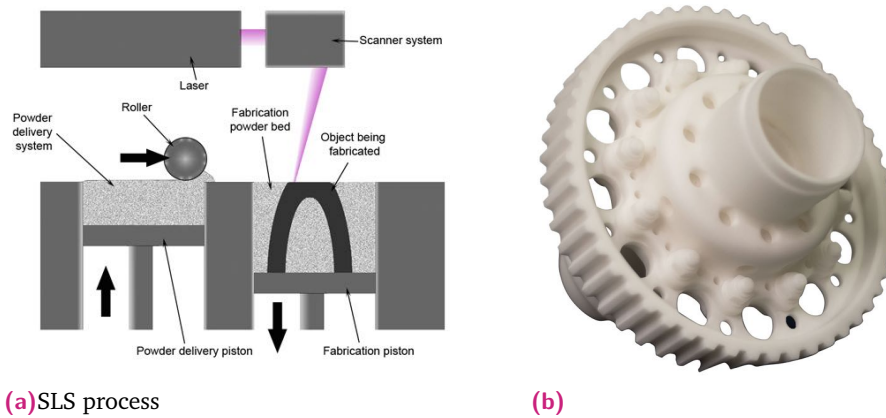
Fig. 4.4.: The Selective Laser Sintering process uses a high-power laser beam that melts and fuses finely powdered material spread on a layer.
