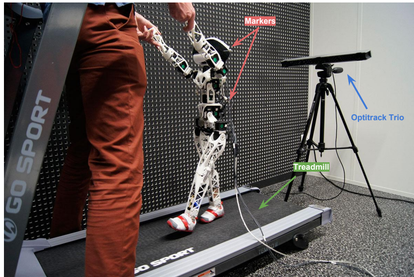
Fig. 8.6.: Proceeding of the walking experiment. Poppy is tracked by an Optitrack trio while it is walking on a treadmill set at 1.8km/h. An expert user provides the sagittal balance needed throughout the experiment.
