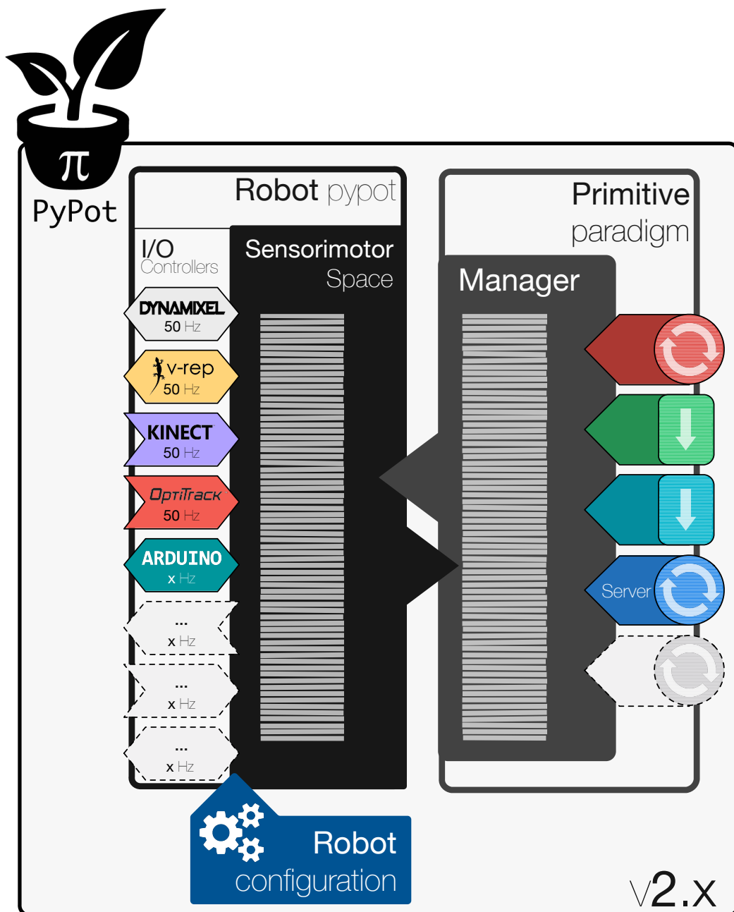
Fig. 7.3.: Diagram showing the modular structure of the pypot library. I/O controllers handle communication with devices while behaviour can be scripted thanks to the primitive paradigms. Between, pypot synchronizes all data and generates easy-to-use accessors.
