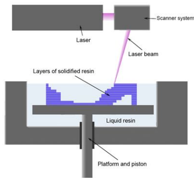
(a) SLA process
