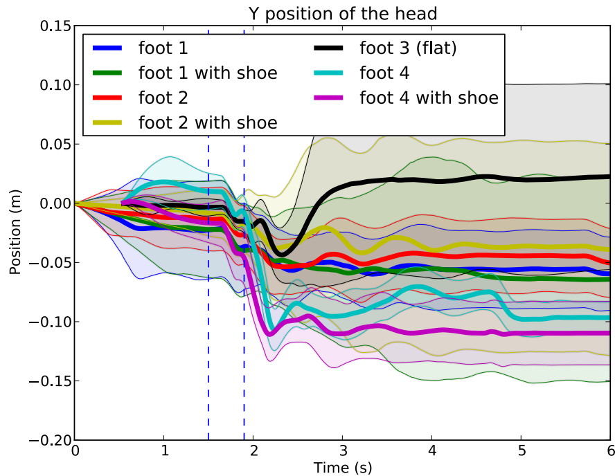
Fig. 8.14.: Evolution of the position of the head in the y axis for each foot tested (see Fig. 8.11 for illustration of each foot).
