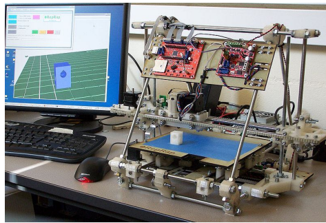
(a) RepRap v2
