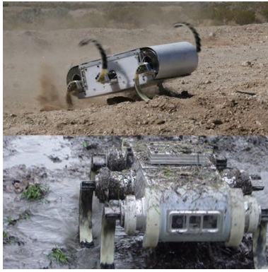
(a) The Rhex robot is a compliant hexapod able to move quickly and robustly over complex terrain.
