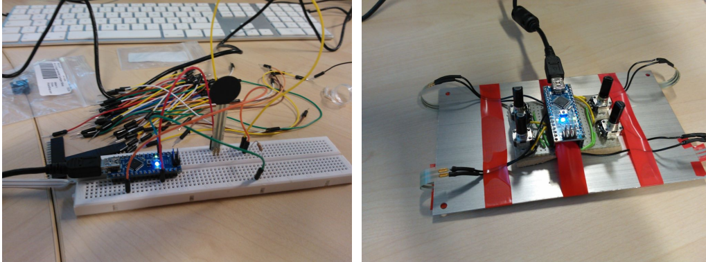
(a) A FSR sensor connected with Arduino nano board. (b) Simple testing assembly with 4 voltage dividers with FSR sensors and potentiometers plugged on an Arduino nano board
