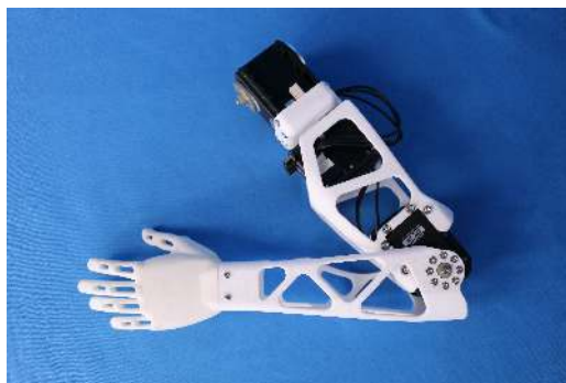
(a) Poppy's arm mechanical structure
