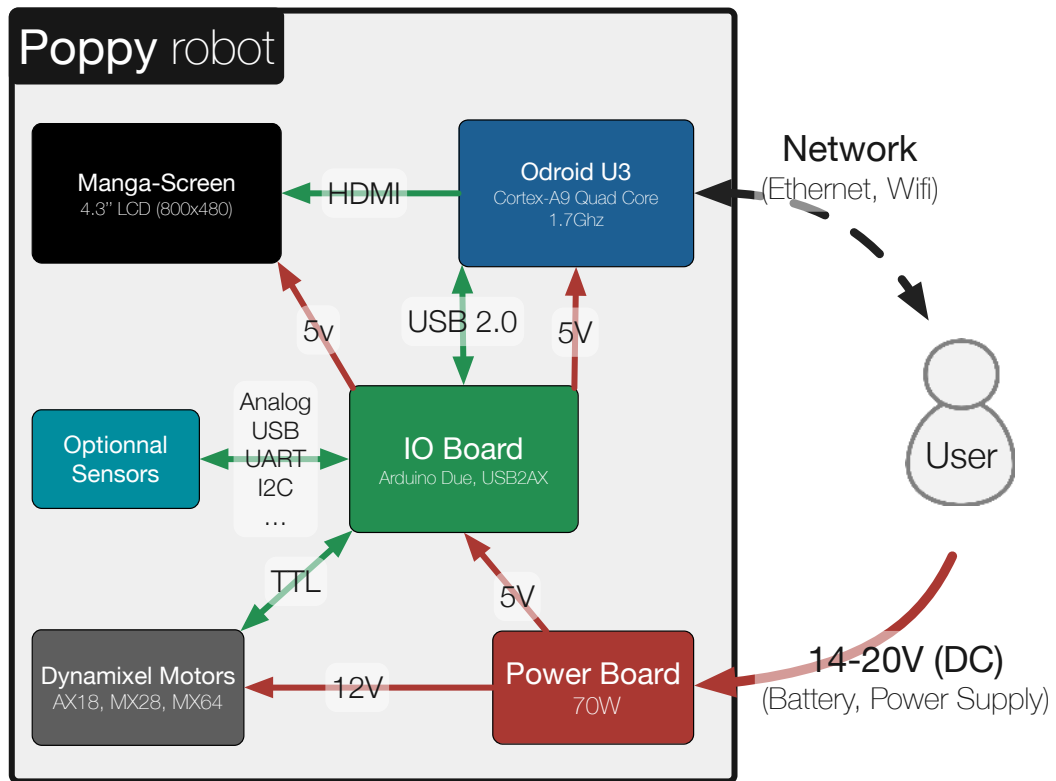
Fig. 6.16.: Overview of the Poppy electronics architecture.
