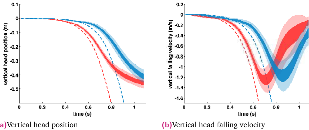
Fig. 8.5.: Results of the single support falling experiment. The blue colour is associated with experiments conducted with bended thighs while the red colour is assigned to straight thighs. For each case, the light colour corresponds to the standard deviation and the dark colour to the 95% confidence interval of the mean value while dashed lines represent theoretical results. These figures show the vertical position (a) and vertical falling velocity (b) of the head of Poppy over time for each case studied. The curve's behaviour change after 800 ms is due to the fact that we catch the robot before it touches the ground.
