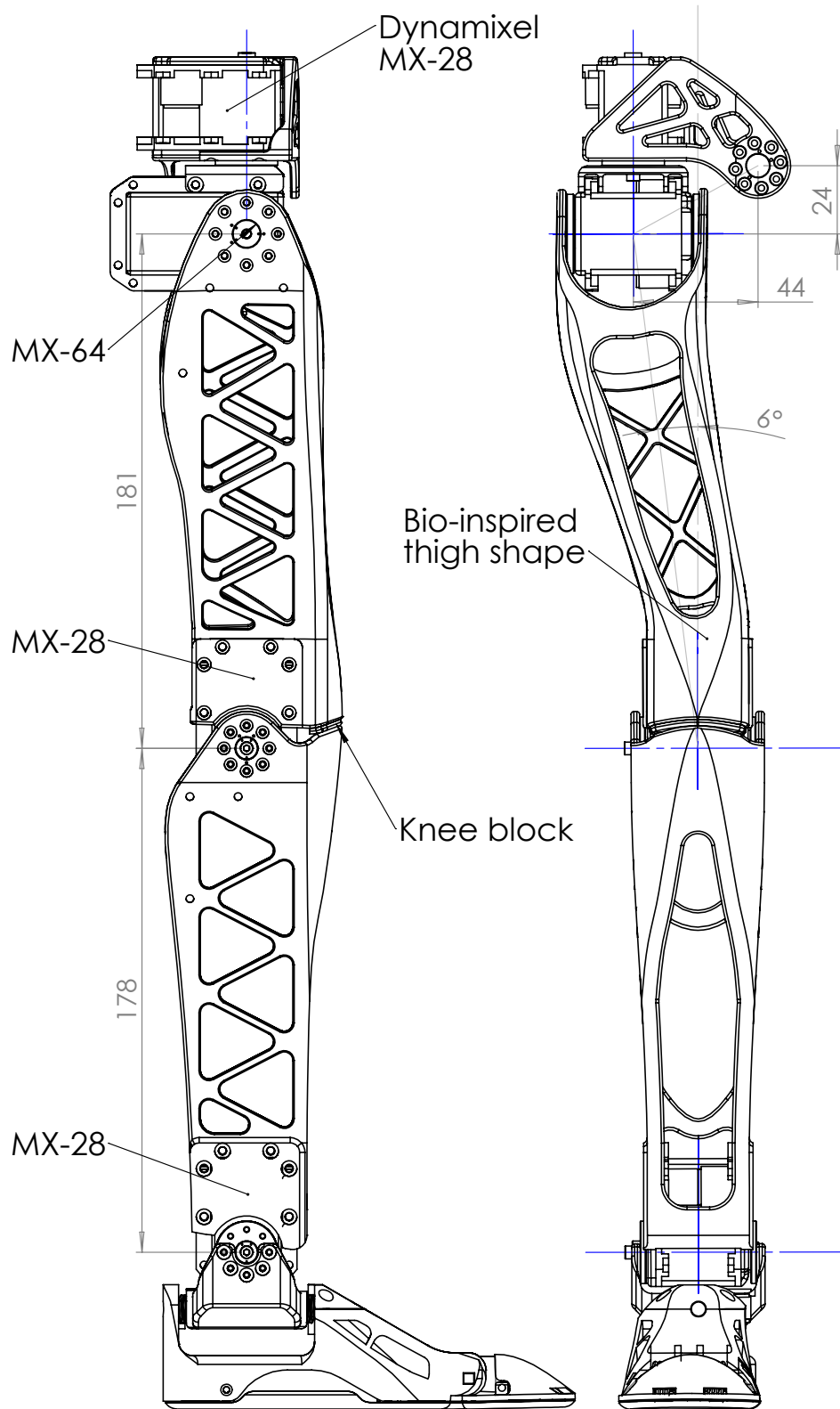
Fig. 6.11.: Blueprint of Poppy's right leg. Parts have a truss structure to reduce the mass, and each leg has 6 DoF. Only the one on the hip use a powerful motors (MX-64), others are powered by MX-28. This choice makes the robot could not support its weight if knees keep bended during walking. Therefore it constraints the research of more human-like gait with straight support leg.
