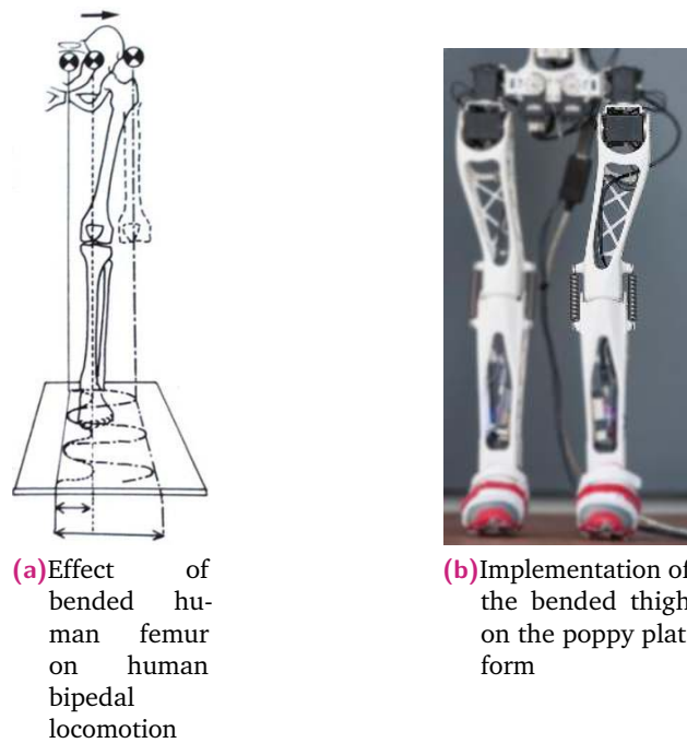
Fig. 8.2.: The human femur is inclined by an angle of 6^\circ , this reduce the distance travelled by the CoG to be supported from one leg to the other during walking. We reproduced it on Poppy and suggest exploring its impact on the robot dynamics.
