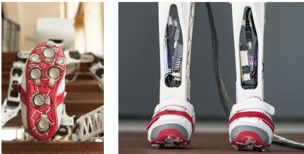
Fig. 8.16.: Physical implementation of the sensors on Poppy. FSR have been placed under feer while Arduino nano board are placed on the leg acquire the data and stream them to the main IO board through USB.
