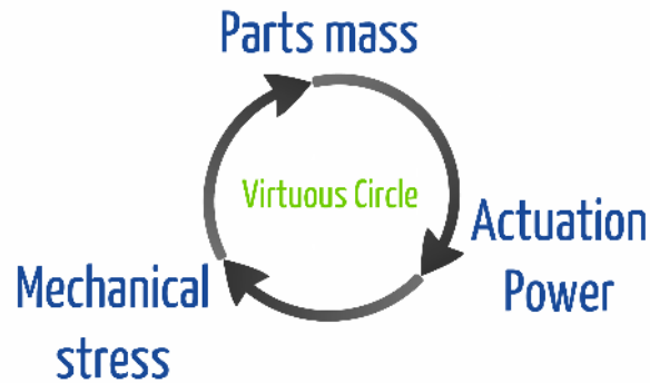
Fig. 6.5.: Using small actuation power reduces the amount of stress applied on the mechanical structure. Thus it is possible to reduce the robustness of mechanical parts by removing matter. Because the global weight is reduced, we can use smaller actuation power, and so on.
