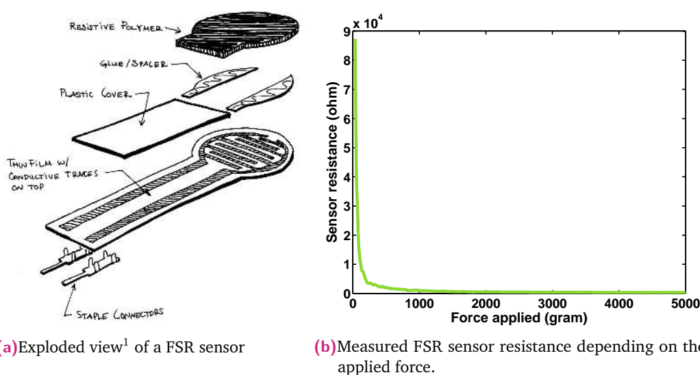
Fig. C.1.: The FSR force sensors are cheap but they have a really non-linear behavior and are not very precise.
