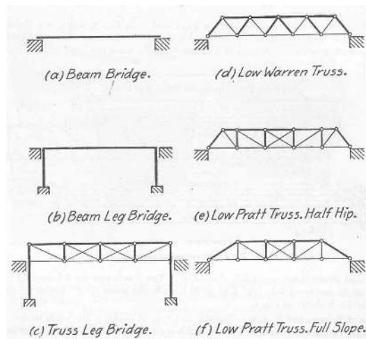
Fig. 6.6.: The truss structure has been massively used in civil engineering, especially to construct bridges. Here is shown several truss structure configurations.
