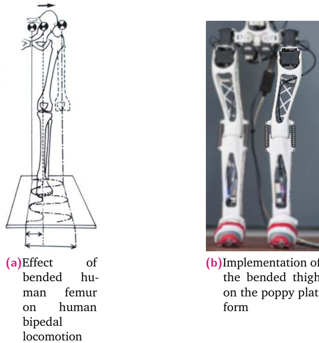
Fig. 8.2.: The human femur is inclined by an angle of 6^\circ , this reduce the distance travelled by the CoG to be supported from one leg to the other during walking. We reproduced it on Poppy and suggest exploring its impact on the robot dynamics.
