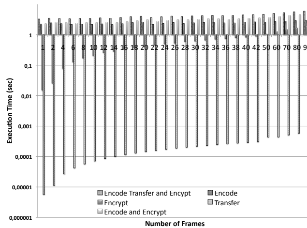
FIGURE 4.12 – Execution times on the hardware
