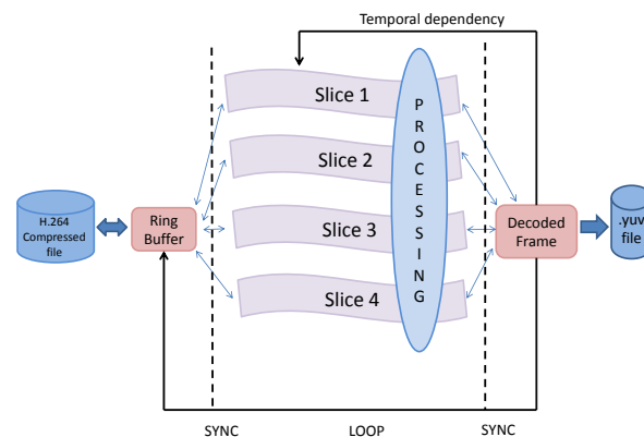
FIGURE 3.19 – Parallelization of the H.264 video decoder
