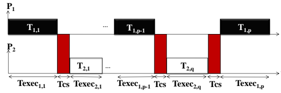
FIGURE 3.10 – Extraction of the context-switch time : Scenario2
