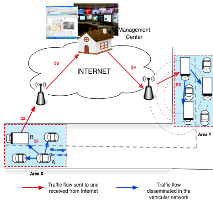
FIGURE 3.1: Multicast in hybrid scenario
