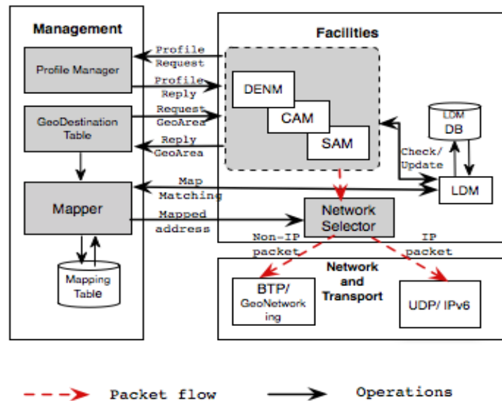
FIGURE 3.5: Framework Integration in the ITS Architecture
