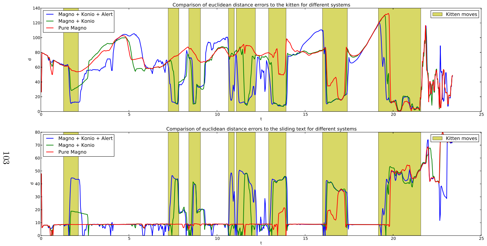
Figure 4.13: Simulation results for all three systems with natural images. The error is computed as the euclidean distance to target, and the yellow areas represent periods at which the kitten moves. (Top) Error against the head of the kitten. (Bottom) Minimal error against the sliding text.
