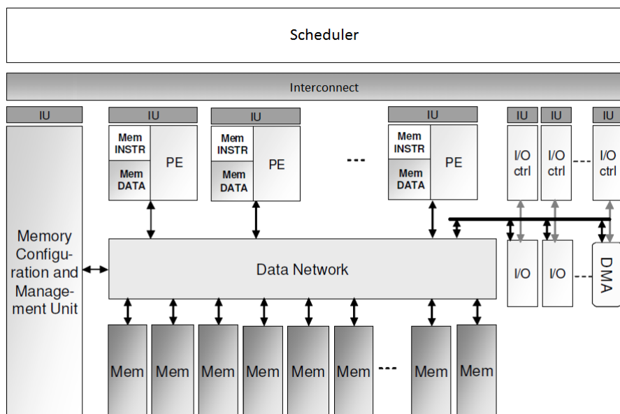
Figure 3.16 – L'architecture SCMP.
