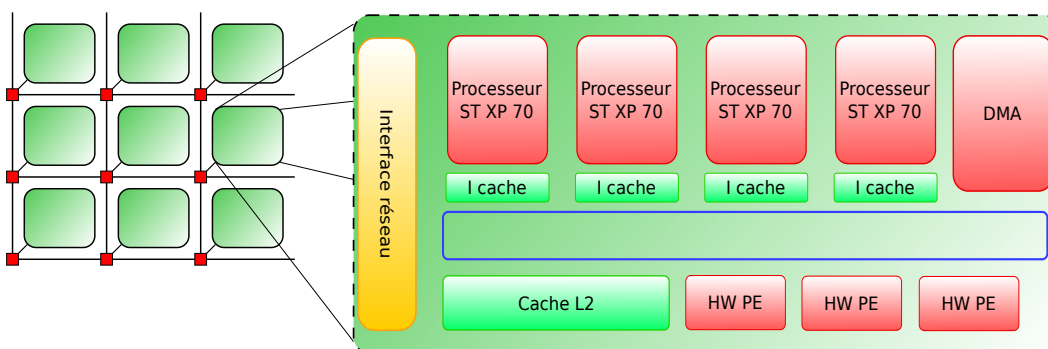
Figure 2.8 – L’architecture P2012.
