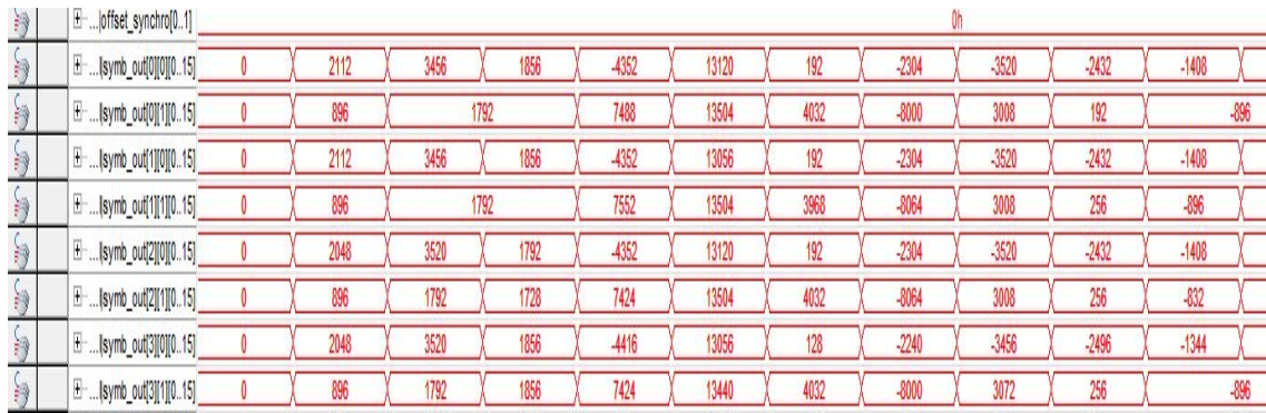
FIGURE 5.19: Altera SignalTap Snapshot of coarse synchronization output of OFDM symbols. Starting from second row, it contains real and imaginary signals alternatively. Correctness of the synchronization is verified by observing that alternate rows have repeating values indicating correct synchronization is achieved.
