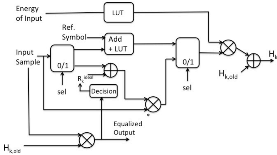
FIGURE 4.10: Channel Estimation and Equalization Architecture which supports both LS and NLMS equalizers
