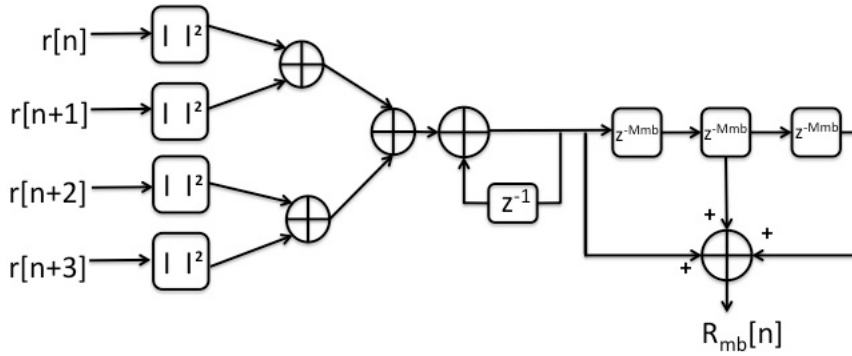
FIGURE 3.18: R = 4 -Parallel Initial Point Energy Computation Block for MBA
