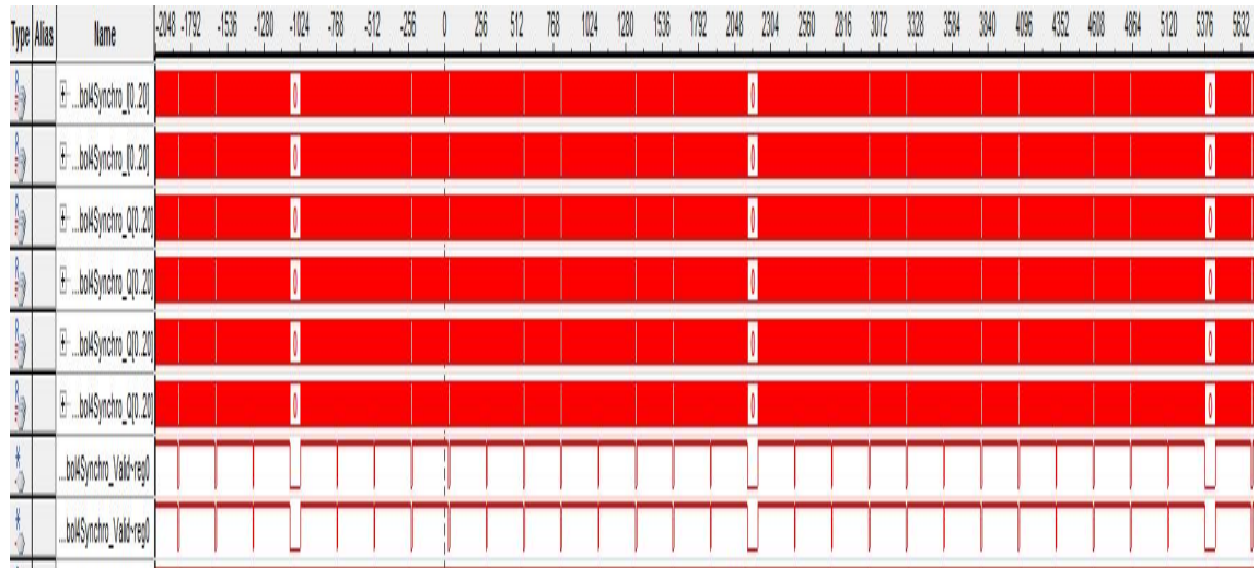
FIGURE 5.18: Altera SignalTap Snapshot of coarse synchronization output. Presence of periodic zeros indicate cyclic prefix removal and bigger gap zeros indicate the removal of the first training symbol in the output fed into FFT block.
