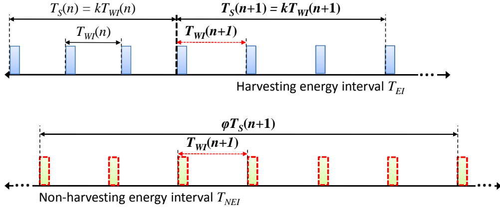
FIGURE 5.3: Positive Energy Power manager. The harvested energy is not only used for the next slot, but also for \varphi slots during T_{NEI} .
