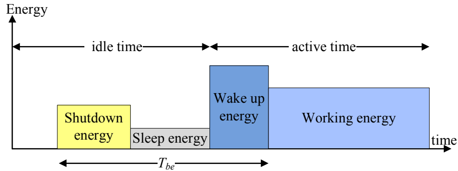
FIGURE 1.1: Break-even time based dynamic power manager. If the idle time is less than T_{be} , the system is not required to shutdown as additional energy to wake-up will be greater than running energy during this period.
