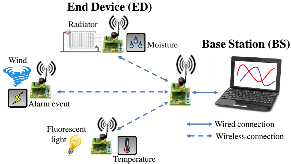
FIGURE 4.1: Single-hop EH-WSN with a base station (BS) and many end device nodes (EDs). All EDs are equipped with a harvested device and a supercapacitor for energy storage. The PM adapts the wake-up interval ( T_{WI} ) of each ED to respect ENO.
