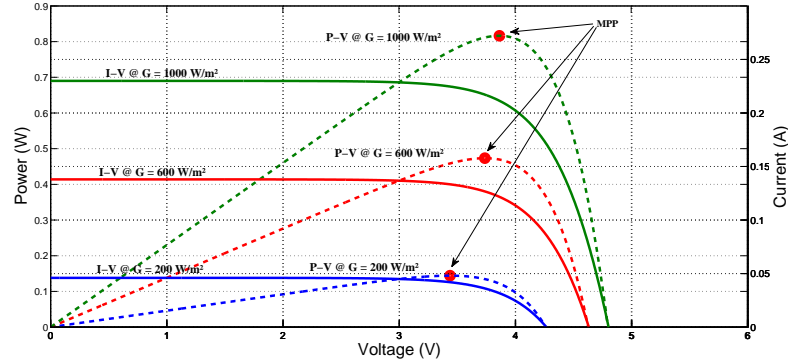
FIGURE 2.1: Maximum Power Point (MPP) of a PV in three different irradiance conditions ( G ) [1]. MPPT mechanism is designed to provide highest power from PVs.
