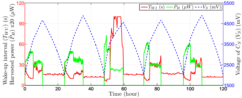
FIGURE 5.14: Adaptations of ED(1) using WVR-PM with \alpha_H = 0.7 .
