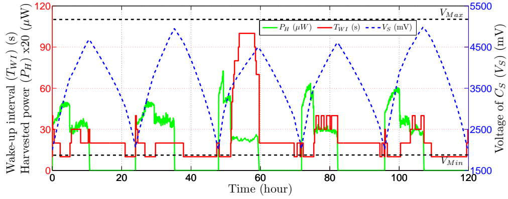
FIGURE 5.17: Adaptations of ED(0) using WVR-PM with \Delta = 10 .
