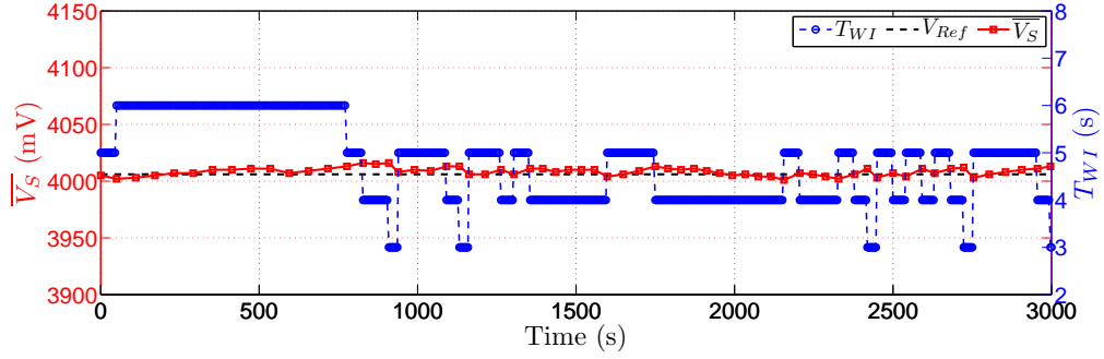
FIGURE 4.7: Voltage of the StoreCap and wake-up interval of the PowWow node when a new super capacitor 0.18F is used.
