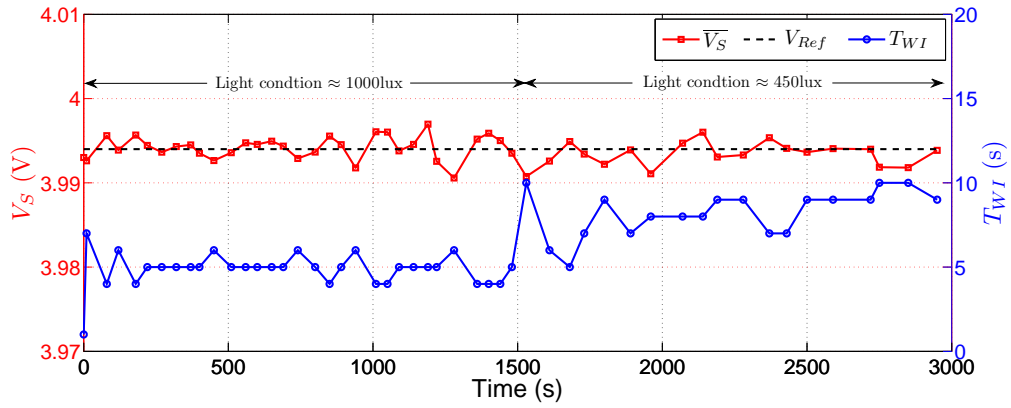
FIGURE 4.5: Voltage of StoreCap when applying EM-PM. \bar{V}_S is fastly converged to V_{Ref} as EM-PM is able to estimate both the harvested and consumed energy.
